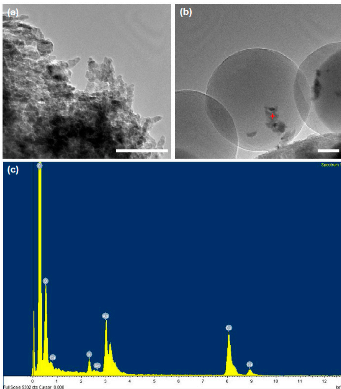
Figure S1. FETEM images of (a) AgNP agglomerates at 1.0 wt% concentration and (b) PS CPhC structures with 1.0 wt% AgNPs (sample C). (c) EDS compositional mapping (Ag) scans from the red cross point of image (b). All scale bars are 20 nm.
