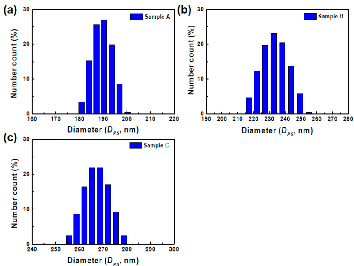
Figure S2. Diameter distribution of PS nanospheres prepared using (a) sample A, (b) sample B, and (c) sample C.
