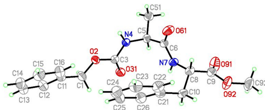
Figure 1. Perspective view of Z-AF-OMe with displacement ellipsoids at the 50% probability level.
