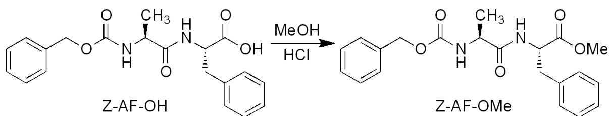
Scheme 1. Acid-catalyzed formation of Z-AF-OMe.
