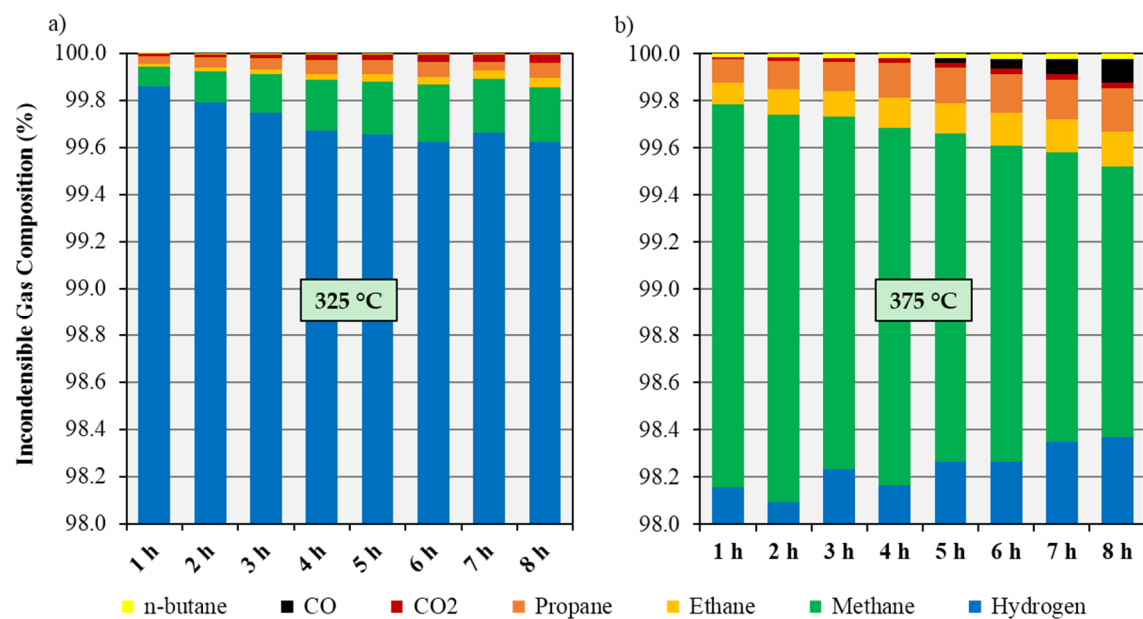
Figure S1. GC analysis of gas samples in the deoxygenation of BG lipids at (a) 325 °C and (b) 375 °C.
