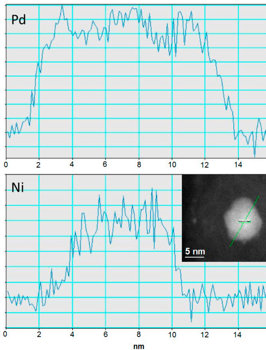
Figure S1. EELS line scan profile for Pd M-edge and Ni L-edge from a single nanoparticle along the scanned line as indicated in the inset.
