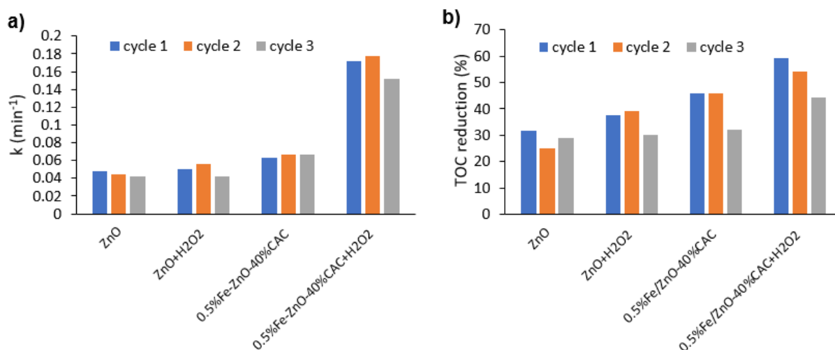
Figure 11. Ibuprofen photocatalytic decomposition (a) and mineralization measured as TOC reduction (b) over ZnO, 0.5%Fe-ZnO-40%CAC and \text{H}_2\text{O}_2 during subsequent photodegradation cycles.
