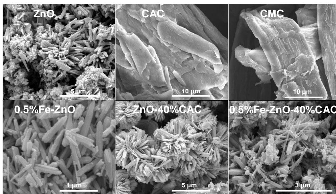
Figure 3. SEM images of selected materials.
