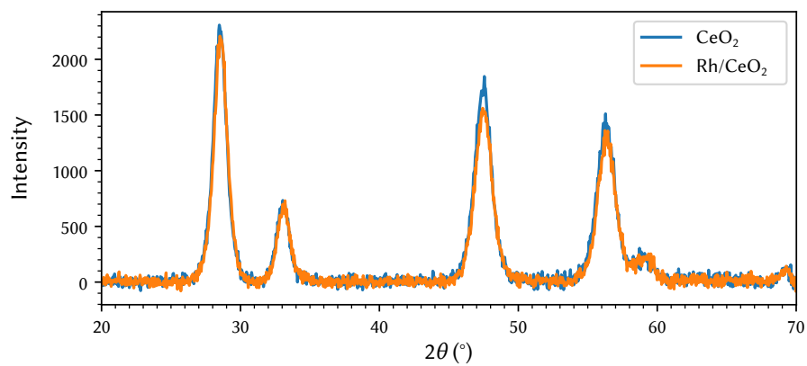
Figure S1: The diffractogram of the CeO 2 , with and without supported Rh, as obtained by the XRD. A background correction was performed on the data to more easily distinguish any formation of new peaks.
