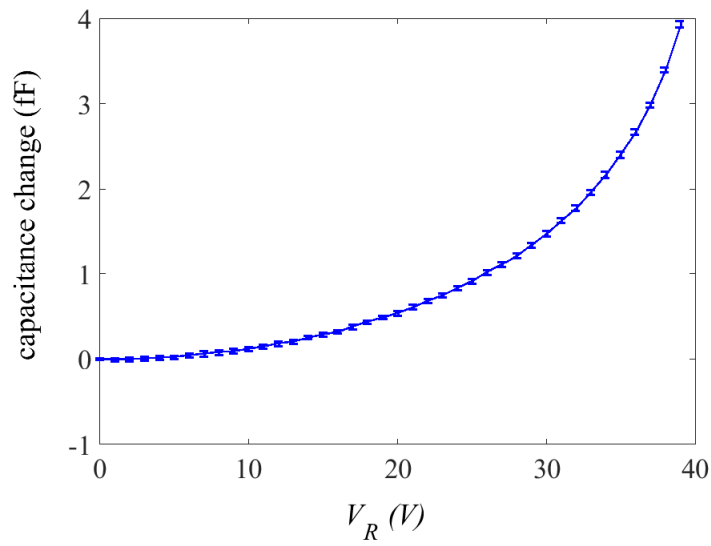
Figure S1. l=20\ \mu\text{m} , RR test configuration; effect of measurement noise on the dispersion (represented through a box-plot) of the experimental response of one device. This plot implies that the measured scattered device responses are primarily governed by the dispersion of the parameters under investigation, and not by measurement errors, see also reference [34] cited in the paper.
