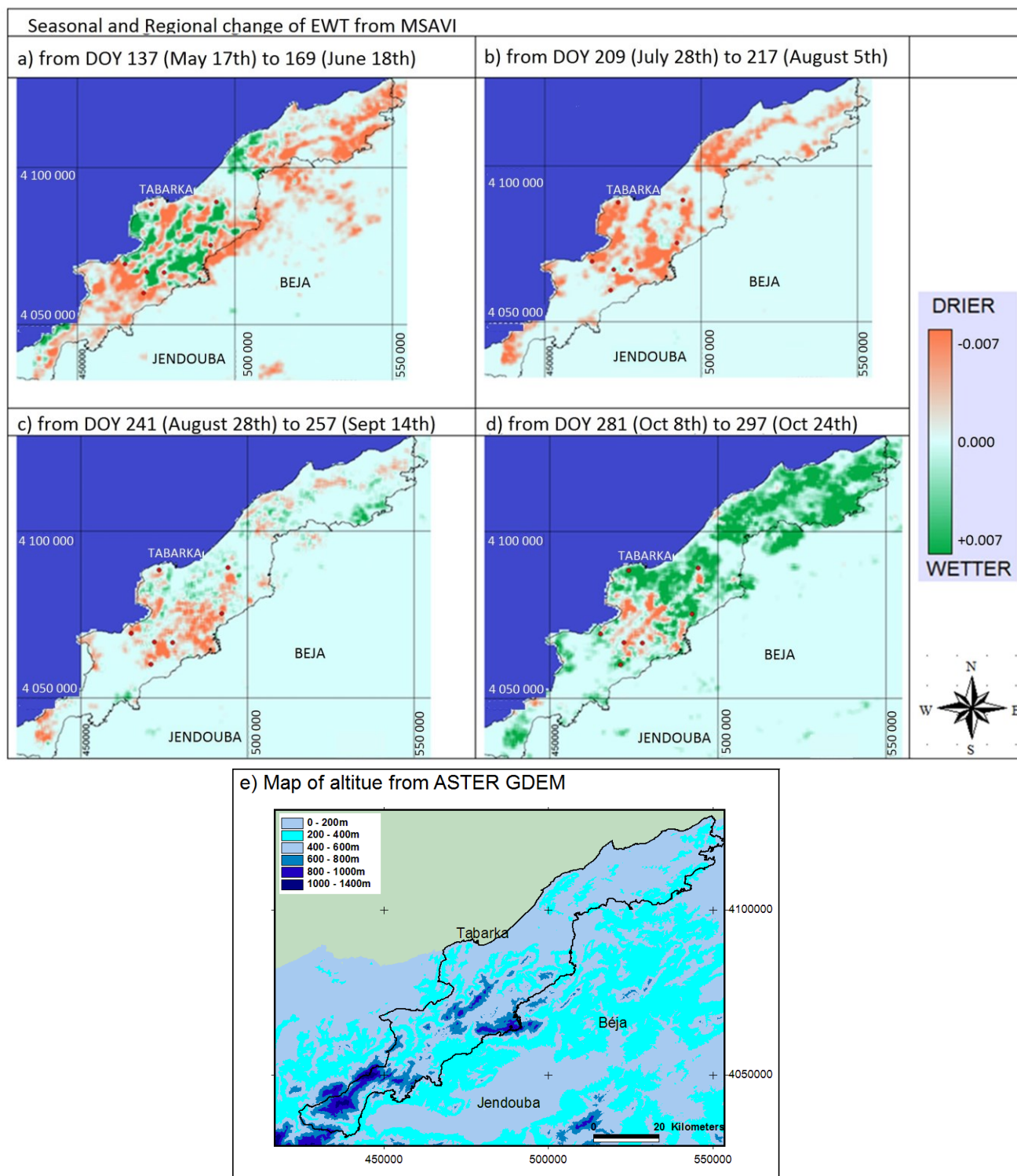
Figure 8. Time course of regional maps of EWT_{CAN} change ( g \cdot cm^{-2} ) in spring ((a); between DOY 137 and 169), mid-summer ((b); between DOY 209 and 217), late summer ((c); between DOY 241 and 257) and early fall ((d); between DOY 281 and 297). Reddish colors indicate drier conditions along the period, and greenish colors indicate wetter conditions along the period. (e) Map of the altitude of the Kroumirie region (processed from ASTER-GDEM).
