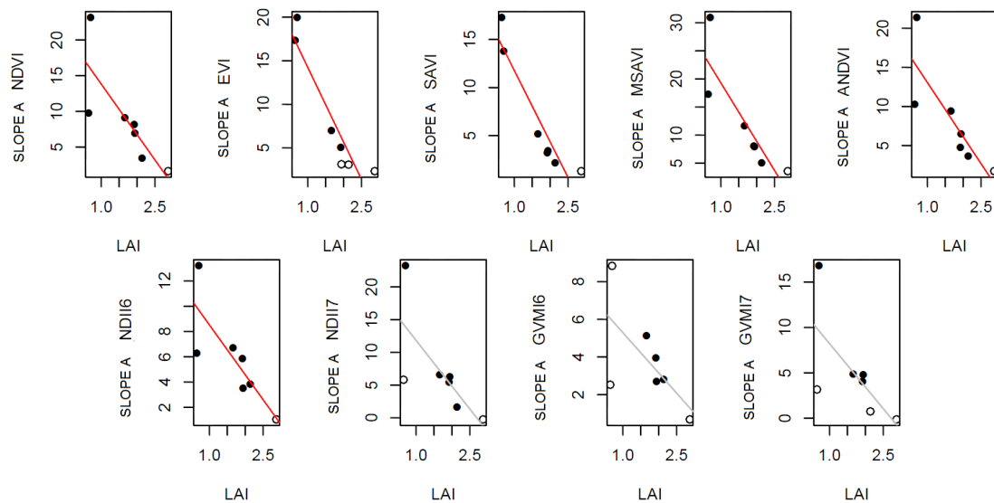
Figure 4. Relationship between LAI plot (X-axis) level and Slope(A) of ( EWT_{CAN} , VI) (Y-axis). (Red line, significant relationship p -value < 0.05 ; grey line, no significant relationship). Black dots represent significant plot-level relationships, and empty dots represent non-significant relationships at the 0.05 threshold for p -values.
