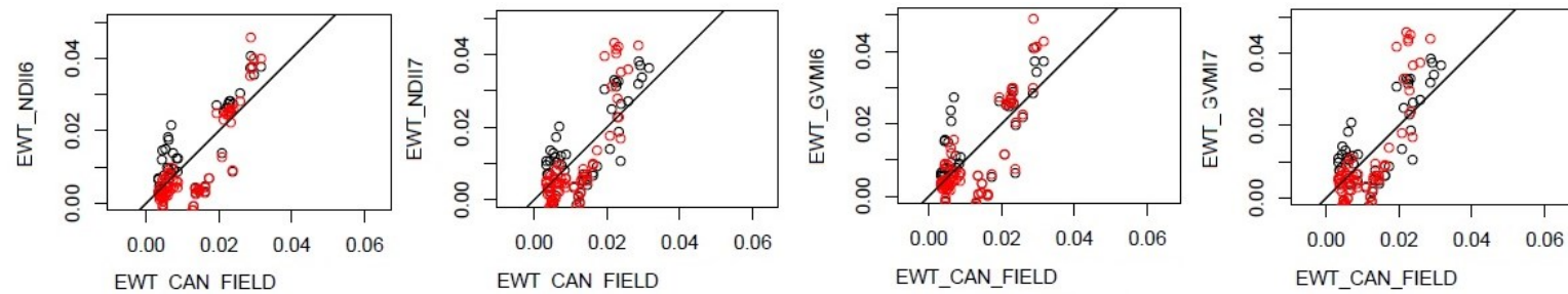
Figure 5. Relationship between EWT_{CAN\_FIELD} from field measurements and modeled EWT_{CAN} from the different VI from MOD1 (black dots) and MOD2 [red dots]). 1:1 line is shown [black line] ( EWT_{CAN} are in g \cdot cm^{-2} ).
