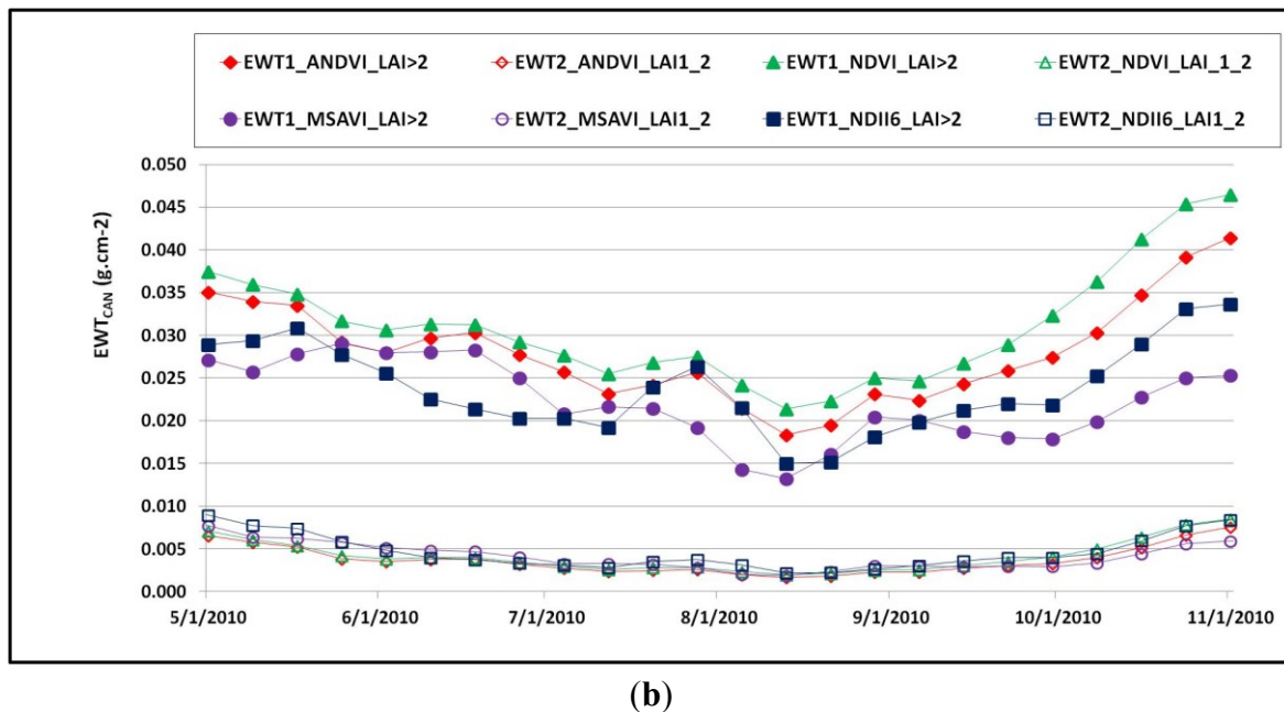
Figure 7. Time course profiles of EWT_{CAN} as estimated from inversion models, MOD1 (EWT1) and MOD2 (EWT2), using the best performing VI over 2010 in the study region. (a) Comparison of MOD1 and MOD2 for herbaceous ( LAI \leq 1 ) and sparse vegetation ( LAI between one and two); (b) comparison of MOD1 and MOD2 for sparse ( LAI between one and two) and dense vegetation ( LAI > 2 ).
