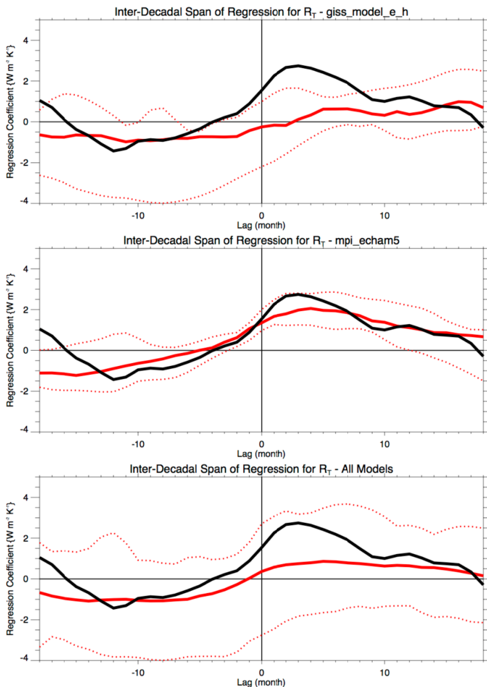
Figure 1. Slope of regression coefficients between monthly temperature anomalies and climate models using (upper) a model which does not accurately reproduce ENSO, (middle) a model which reproduces ENSO reasonably well, and (bottom) all CMIP3 models. Black lines are from observations, red lines are results averaged by decade, and red dashed lines indicate the range of model results.
