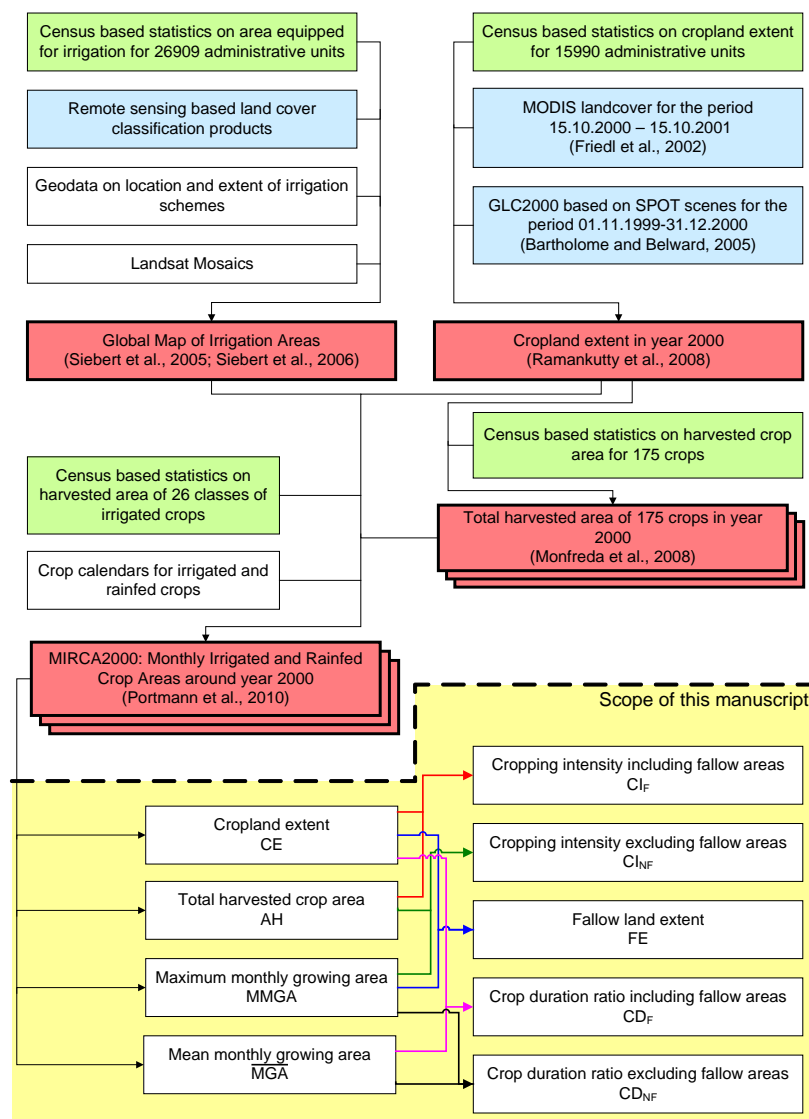
Figure 1. Information flow diagram showing (1) major input datasets used to generate the MIRCA2000 dataset (above the dotted line), and (2) processing of the MIRCA2000 data to compute cropping intensities, fallow extent and crop duration ratios (below the dotted line on yellow background). Red boxes indicate global grid data at 5 arc-minute resolution, blue boxes represent land cover classification products based on remote sensing and green boxes indicate statistical information derived from census based inventories.
