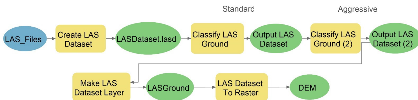
Figure 3. Workflow shown in ArcGIS Pro ModelBuilder for ground classification of LiDAR point clouds and generation of a digital elevation model.
