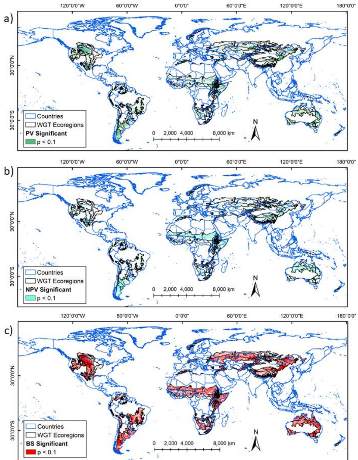
Figure S2. Areas within the WGT exhibiting significant trends at p < 0.1 for a) F_{PV} ; b) F_{NPV} ; and c) F_{BS} .
