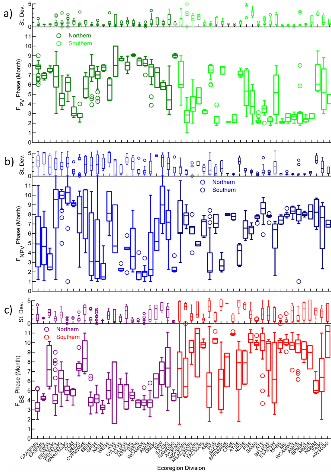
Figure S4. Fence box plots showing the median, upper and lower hinges and upper and lower fences of the average phase (month of maximum amplitude) of the cosine curve fitted to the time series of a) F_{PV} , b) F_{NPV} and c) F_{BS} for 2001 – 2018 within WGT Divisions (listed in Table A1).
