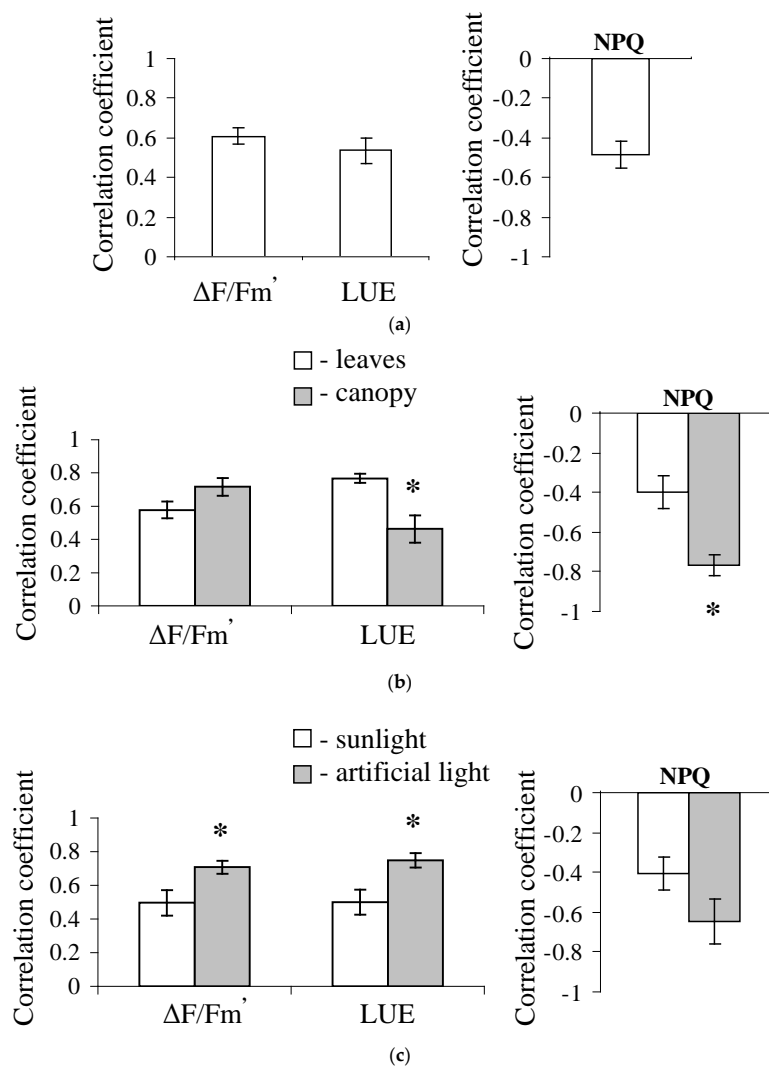
Figure 2. The connection of PRI with the quantum yield of photosystem II ( \Delta F/F_m' ), nonphotochemical quenching (NPQ), and light use efficiency (LUE). (a) Average correlation coefficients of PRI with \Delta F/F_m' ( n = 110 ), LUE ( n = 63 ), and NPQ ( n = 50 ); (b) Average correlation coefficients of PRI with \Delta F/F_m' , LUE, and NPQ for measurements of the photochemical reflectance index in leaves ( n = 86 , n = 15 , n = 38 , respectively) and canopy ( n = 24 , n = 48 , n = 12 , respectively); (c) Average correlation coefficients of PRI with \Delta F/F_m' , LUE, and NPQ with measurements under sunlight ( n = 52 , n = 54 , n = 33 , respectively) or artificial light ( n = 58 , n = 9 , n = 17 , respectively). * the groups significantly differed from another one ( p < 0.05 , Student's test).
