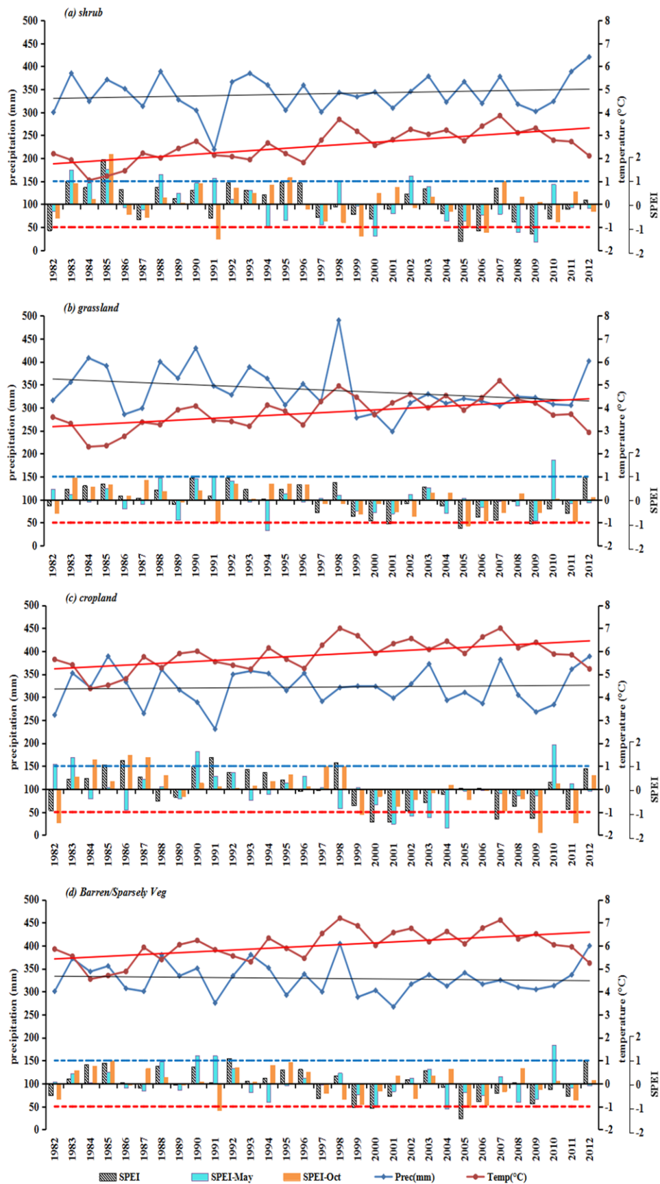
Figure S2. Meteorological metrics analysis during 1982-2012 among different land cover types. All the data are spatial average value for a specific land cover type.
