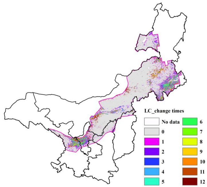
Figure S1. The variation of MODIS land cover types during 2001-2012
