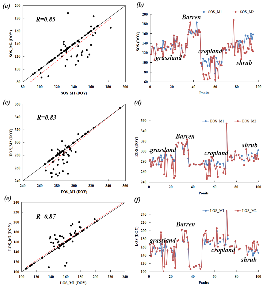
Figure S3. Comparison phenology metrics between threshold and derivation method. M1, M2 means dynamic threshold method and derivation methods, respectively. Black line in a, c, e is 1:1 line, and red dotted line is correlation slope. 100 points was selected randomly at four land cover types, which showed in b, d, f.
