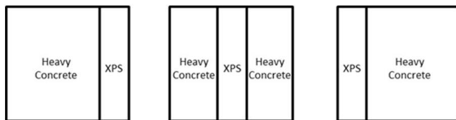
Figure 1. Walls' stratigraphy.
