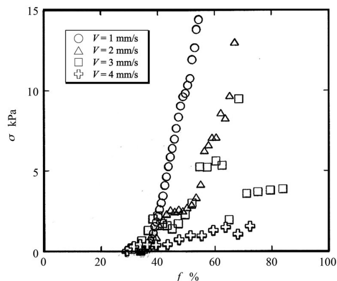
Figure 15. Compression stress vs. snow fraction by constant velocity compression test. Imitation fresh snow ( d_p = 1 mm).
