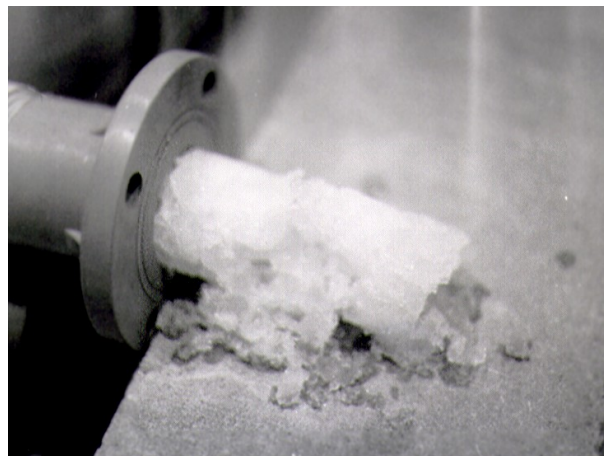
Figure 6. Snow noodle formed at porous wall in a water separator.
