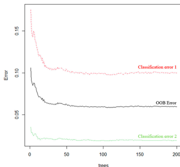
Figure 3. OOB Errors.
