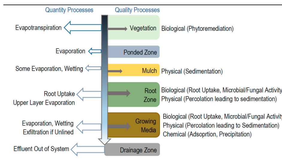
Figure 1. Schematic of vegetated LID metal remediation processes.
