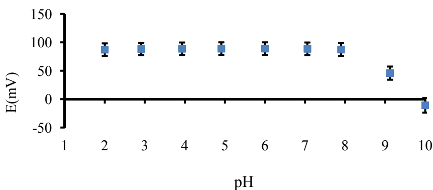
Figure 4. Effect of pH on the potential response of lidocaine sensors. Mean \pm SD values are shown ( n = 3 ).
