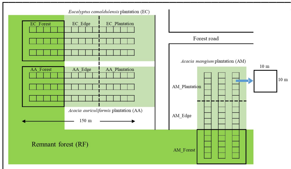
Figure 2. The layout of three transect lines of 10 m × 150 m set up along the forest remnant (Forest, –50 m to 0 m) through forest–plantation edge (Edge, 0 m to 50 m) and plantation stand (Plantation, 50 m to 100 m) in three exotic plantations: Eucalyptus camaldulensis (EC), Acacia auriculiformis (AA), and A. mangium (AM).
