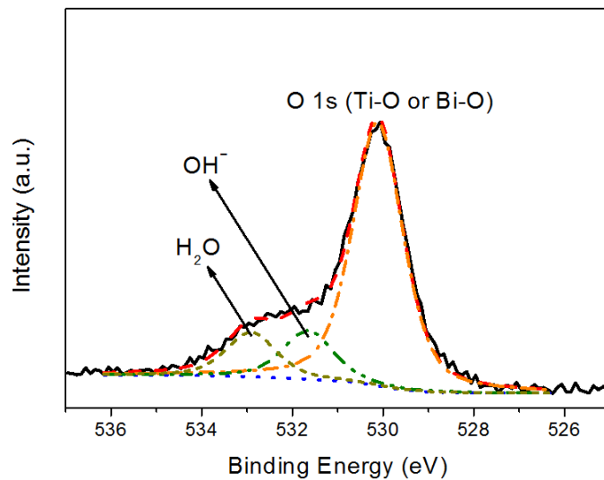
Figure 5. O 1s XPS spectrum recorded from the coating.
