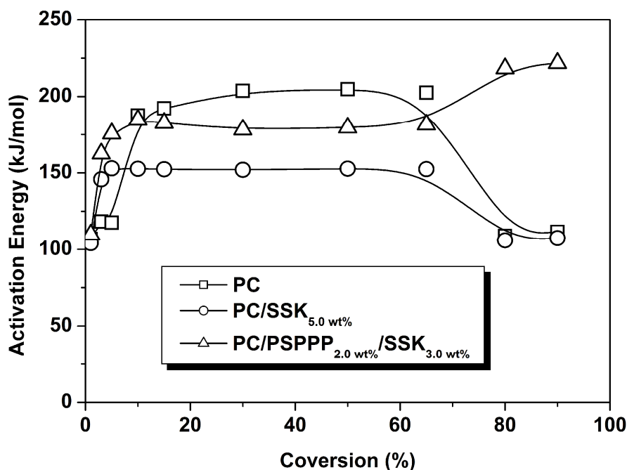
Figure 1. Activation energy ( E_a ) curves of neat PC and flame retardant PCs calculated according to Flynn method [35].
