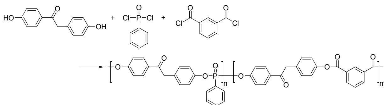
Scheme 7. Synthesis route of BHDB-poly(arylate- co -phosphonate) (PAL- co -PPN).
