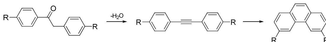
Scheme 6. Potential route to aromatization of BHDB segments.
