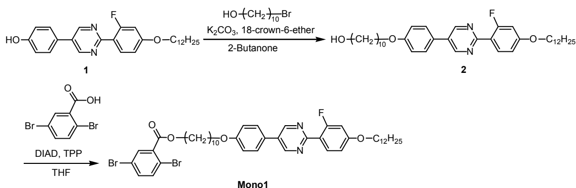
Scheme 1. Synthesis of monomer bearing LC moiety.
