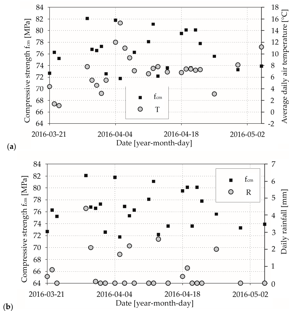
Figure 4. Laboratory test results for concrete mix CM_B type: (a) compressive strength and corresponding average daily air temperatures; (b) compressive strength and corresponding daily rainfall.
