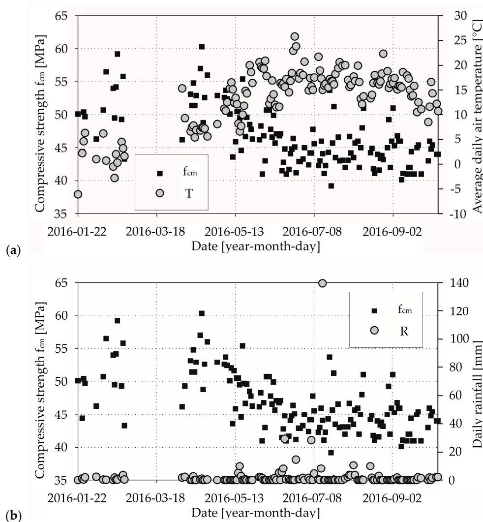
Figure 2. Laboratory test results for concrete mix CM_A type: (a) compressive strength and corresponding average daily air temperatures; (b) compressive strength and corresponding daily rainfall.
