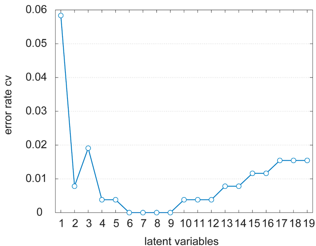
Figure S2. Error rate as a function of latent variables calculated in the PLS-DA model for HDPE and LDPE classification. 6 LVs is the optimal number.
