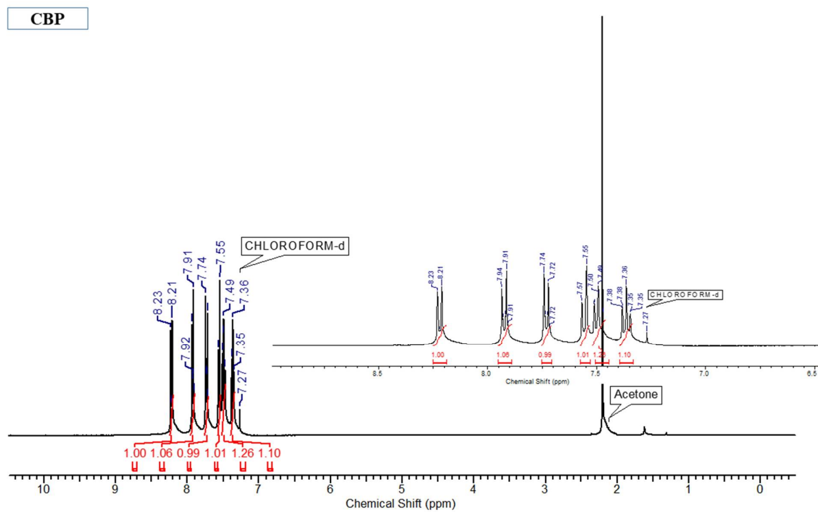
Fig. S1 ^1\text{H} NMR analysis of 4,4'-Bis(9-carbazolyl)-1,1'-biphenyl,4,4'-N,N'-Dicarbazole-1,1'-biphenyl (CBP)
