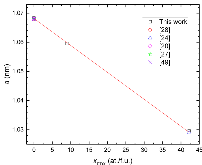
Figure 3. Lattice parameter a vs. the Si content in the clathrate phase x_{\text{EDX}} . The lattice parameters of the ternary clathrates of similar compositions from the literature are included for comparison.
