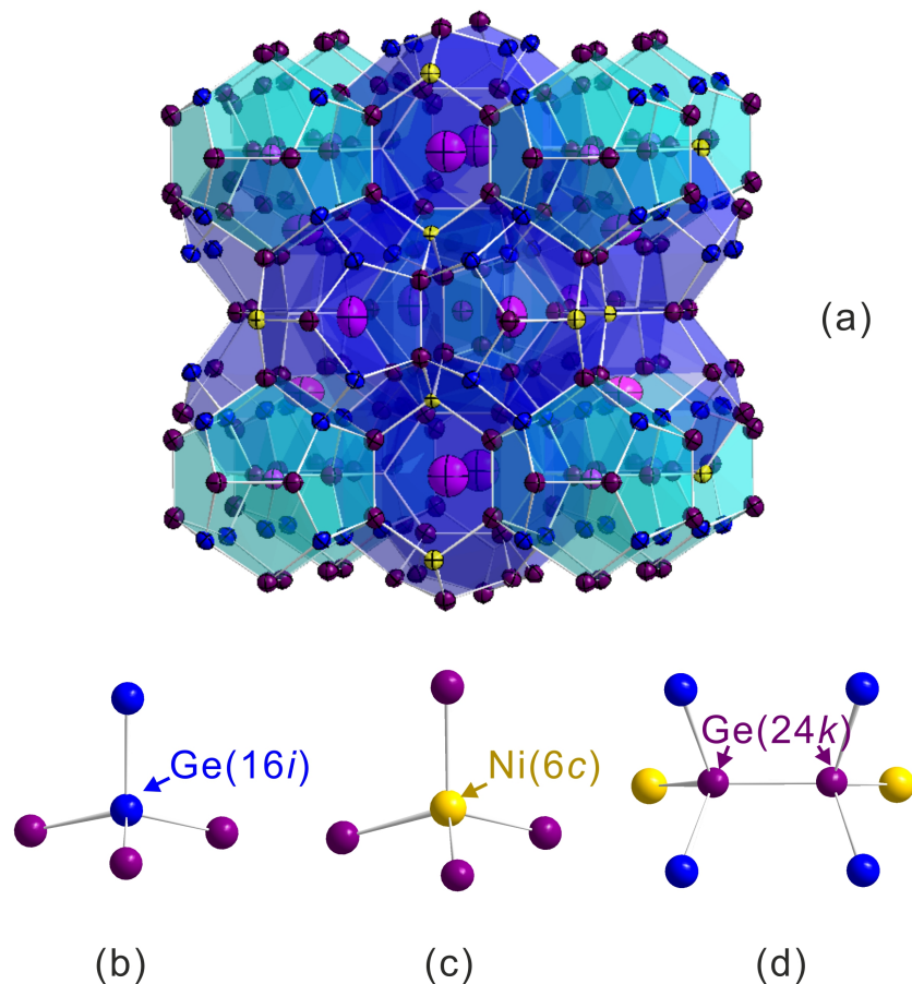
Figure 4. Crystal structure of type-I clathrate (a) and atomic environment (tetrahedral bonds) in different sites (b) Ge(16i); (c) Ni(6c); and (d) Ge(24k).
