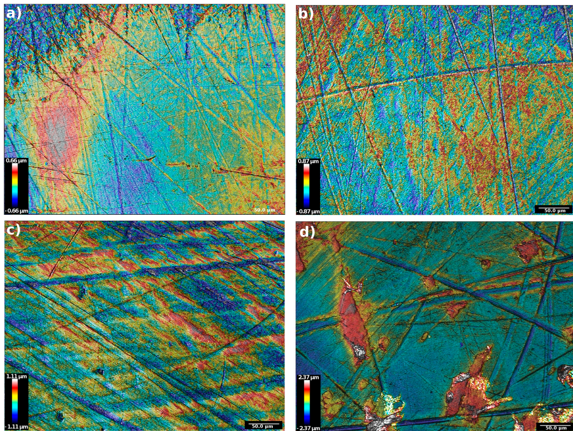
Figure S1 – Supplementary figure with a second set of contour images of the topographies acquired on the worn inner surfaces of four loaded specimens: a VE; b STD; c XL-75; d XL-50. The observations are very similar to the ones described for Figure 4.
