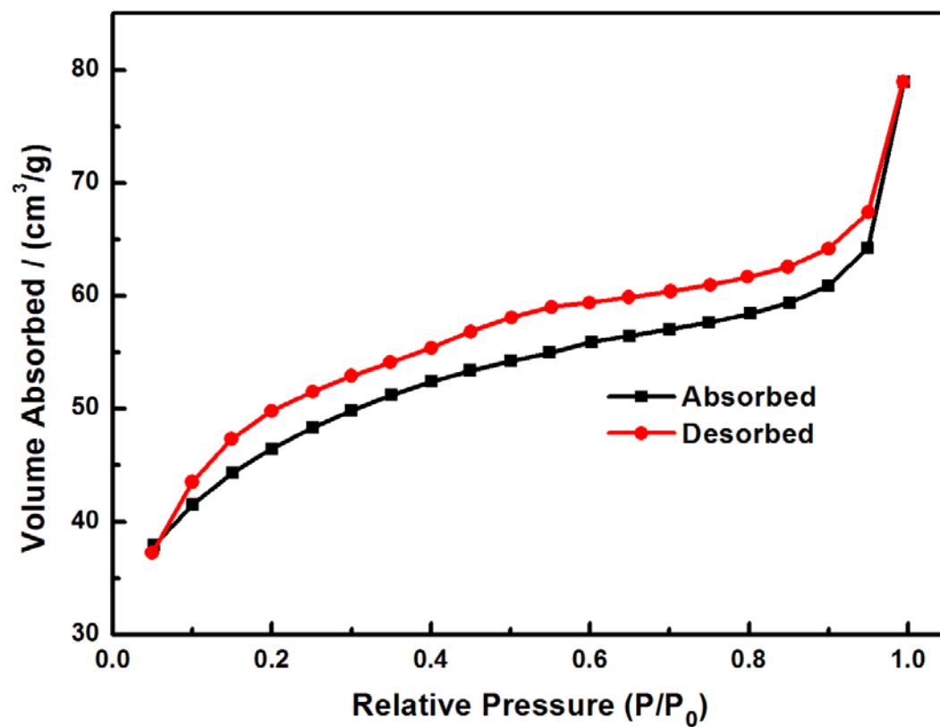
Figure S3. Adsorption and desorption curve of BCN sheets (BET surface area: 158 m 2 /g)
