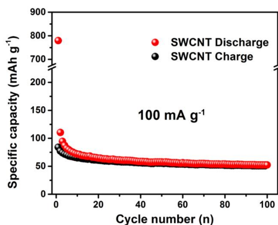
Figure S1. Cycling performance of the pure SWCNT electrode for SIBs at a current density of 100 mA g -1 .
