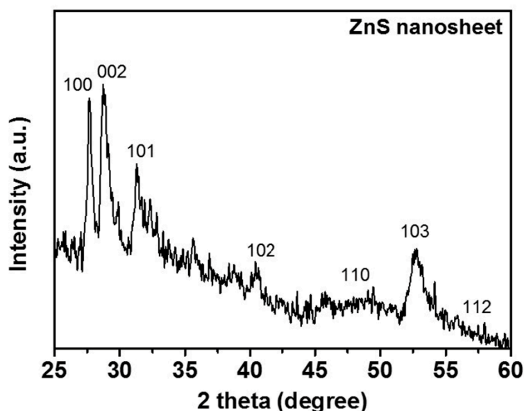
Figure S1. The XRD characterization of the ZnS nanosheet.
