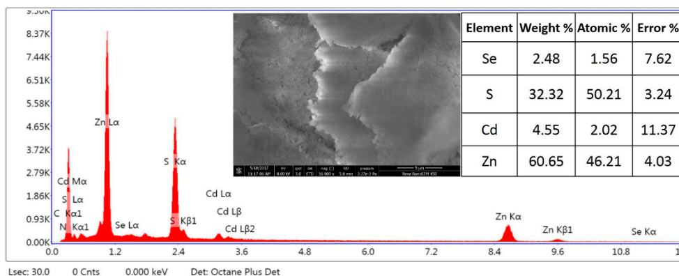
Figure S2. The EDX measurement of the QD-ZnS NIAM (inserted images show the SEM pattern of the QDs-ZnS NIAM sample and the test data).
