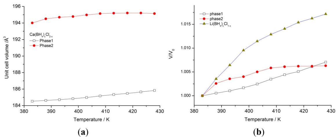
Figure S3. (a) Temperature dependency of lattice parameters of phase 1 and 2; (b) Normalized unit cell volumes.
