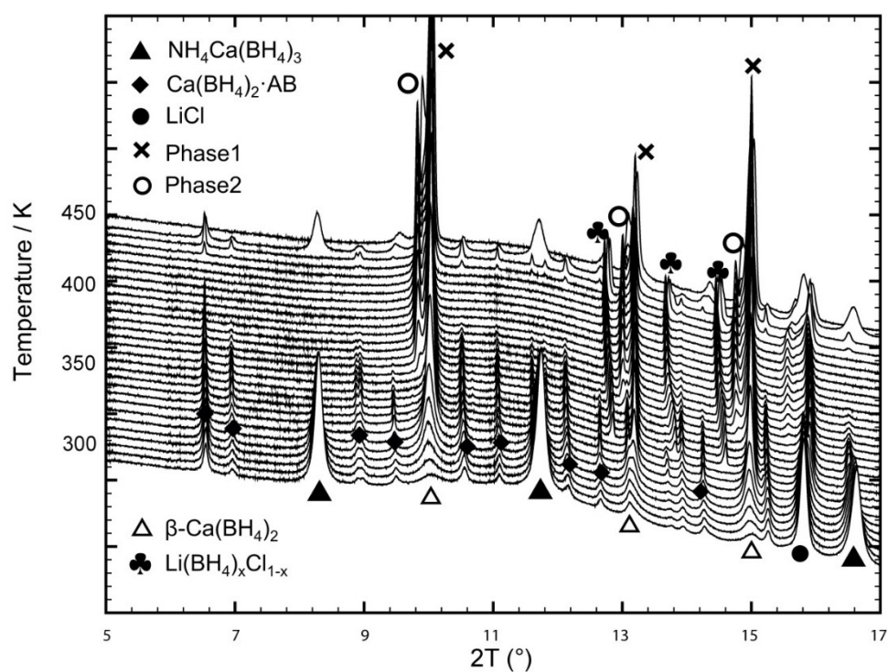
Figure S1. In-situ synchrotron X-ray powder diffraction data as function of temperature for the chloride based sample 1:1:1.
