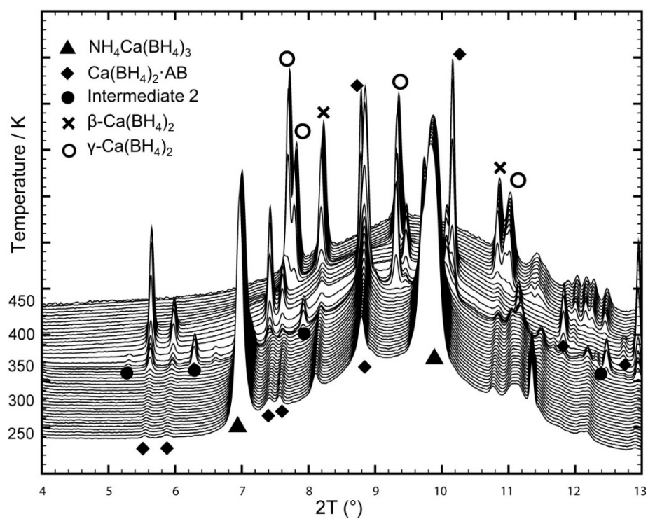
Figure S1. In-situ synchrotron X-ray powder diffraction data as function of temperature for the chloride based sample 1:1:1.
