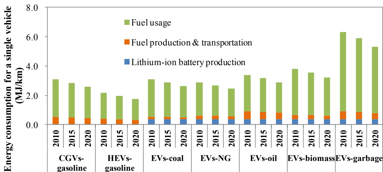
Figure 2. Energy consumption for a single vehicle (HEVs-gasoline means the hybrid electric vehicles using gasoline, EVs-fuel means the electric vehicles using the electricity generated by fuel combustion).
