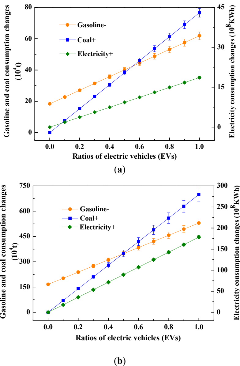
Figure 4. The consumption changes of gasoline, coal and electricity under different ratios of electric vehicles in China (“+” represents increase, “−” represents reduction): (a) 2015 and (b) 2020.
