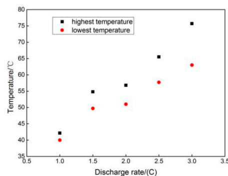
Figure 2. Battery surface temperature at different discharge rates.
