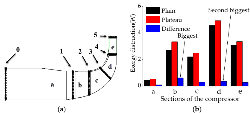
Figure 15. Exergy destruction comparison analysis: (a) Sections of the compressor passage; (b) Exergy destruction in the compressor.
