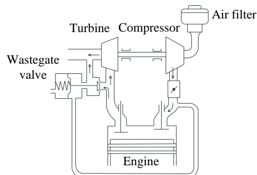
Figure 1. Principle of turbocharged engine.
