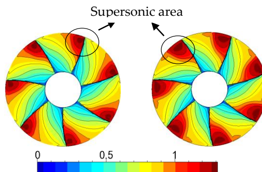
Figure 7. Relative Mach number distribution at the inlet of the impeller ((left) 0 m, (right) 4500 m).
