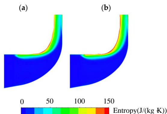
Figure 9. Entropy distribution of meridional averaged plane ((a): plain; (b): plateau).
