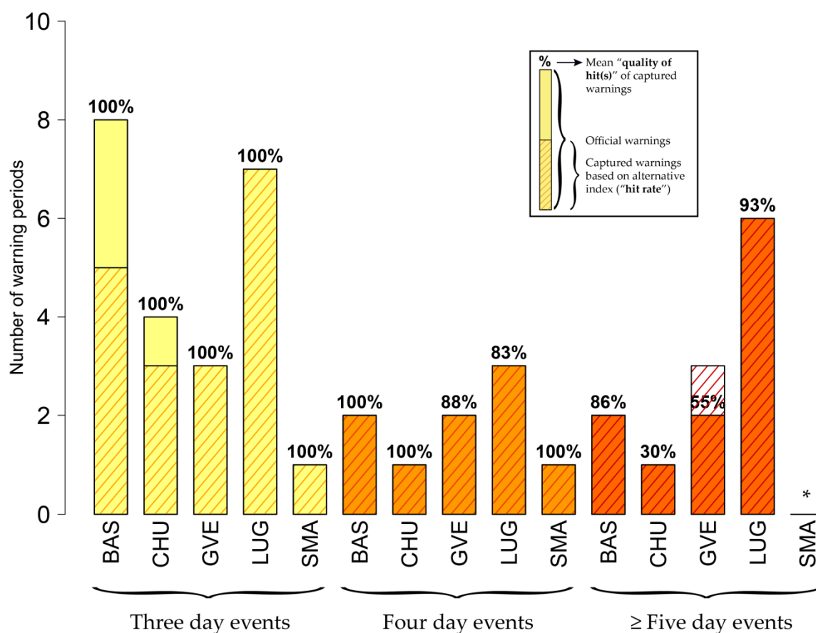
Figure S1. As Figure 10 but for wbgt.shade .
