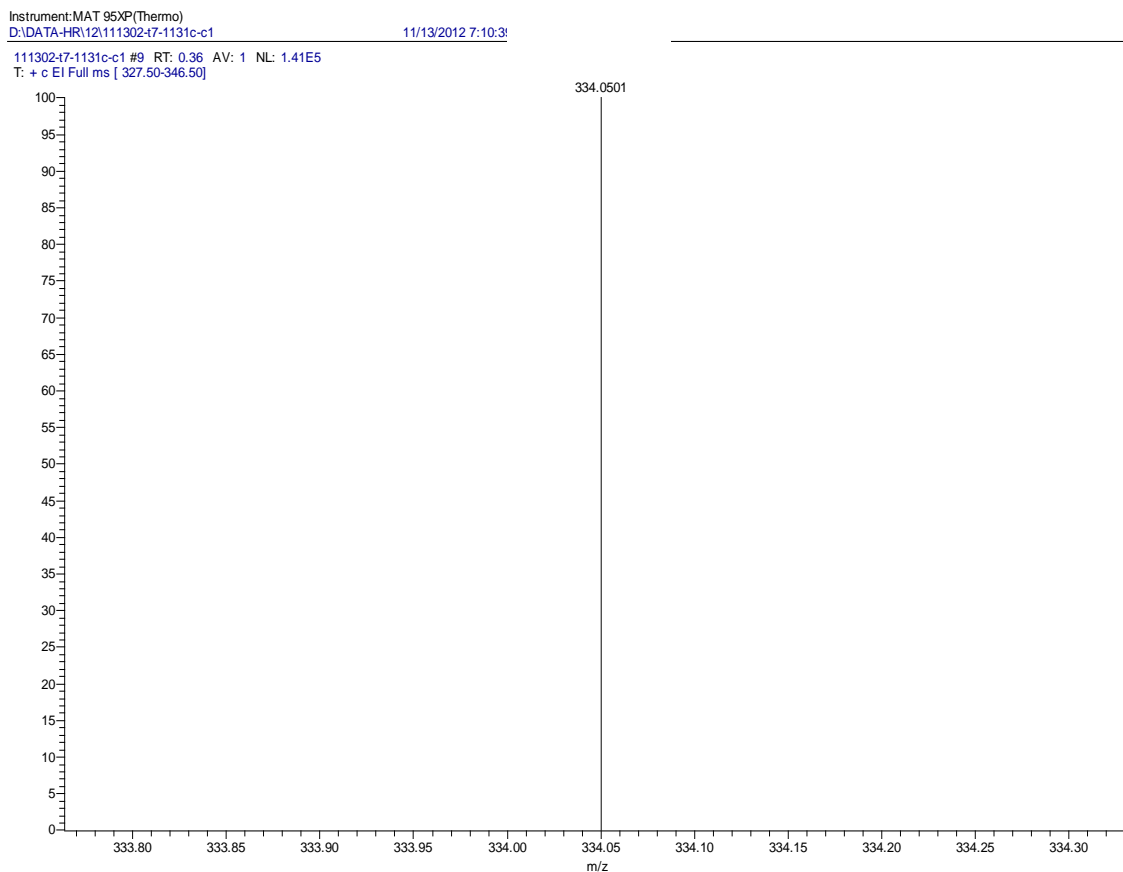
Figure S2. HR-EIMS of compound 1.
