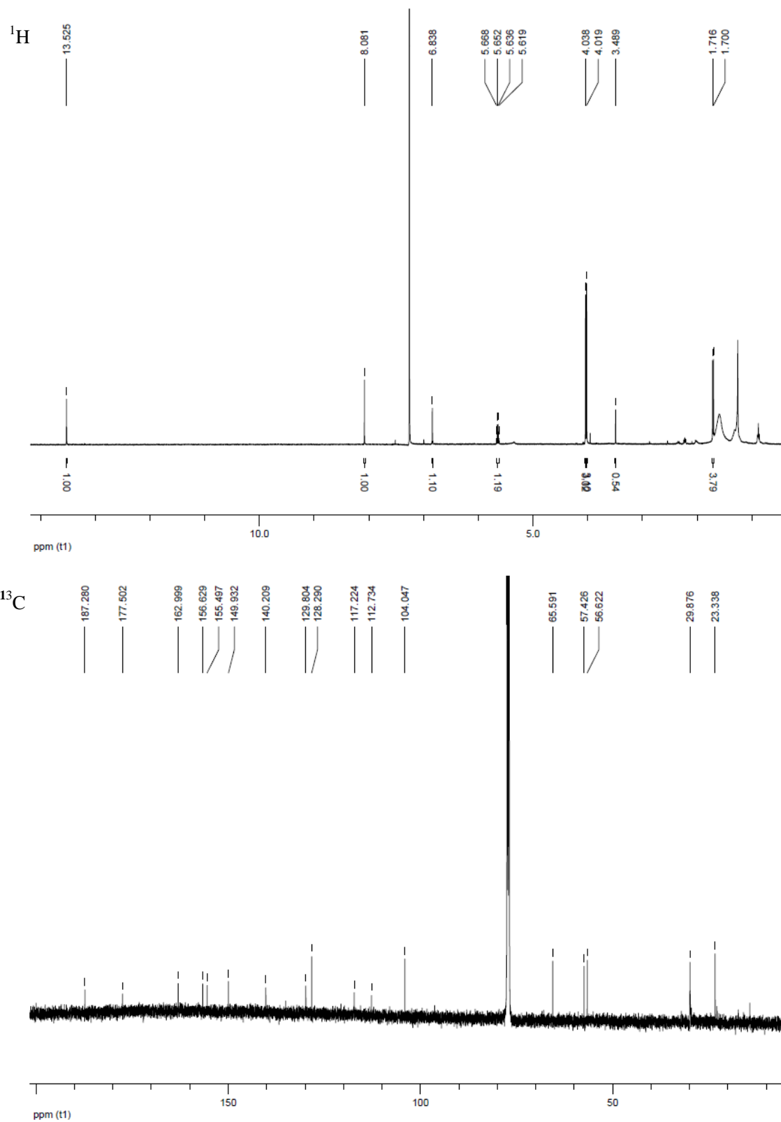
Figure S1. ^1\text{H} , ^{13}\text{C} , Dept 135, Dept 90, ^1\text{H} - ^1\text{H} cosy, HMQC, HMBC of compound 1.
