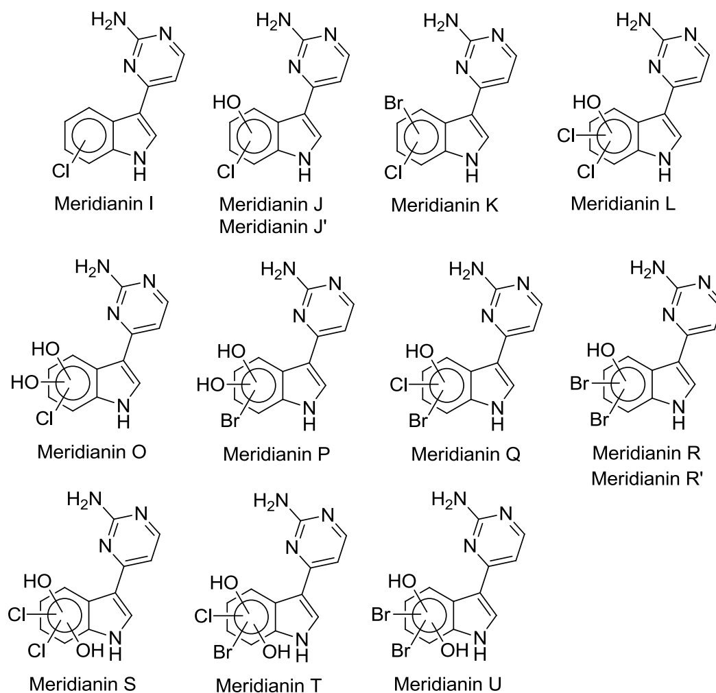
Figure S1. Proposed chemical structures of the new minority meridianins I–U detected by LC-HRMS/MS from Aplidium falklandicum 1.
