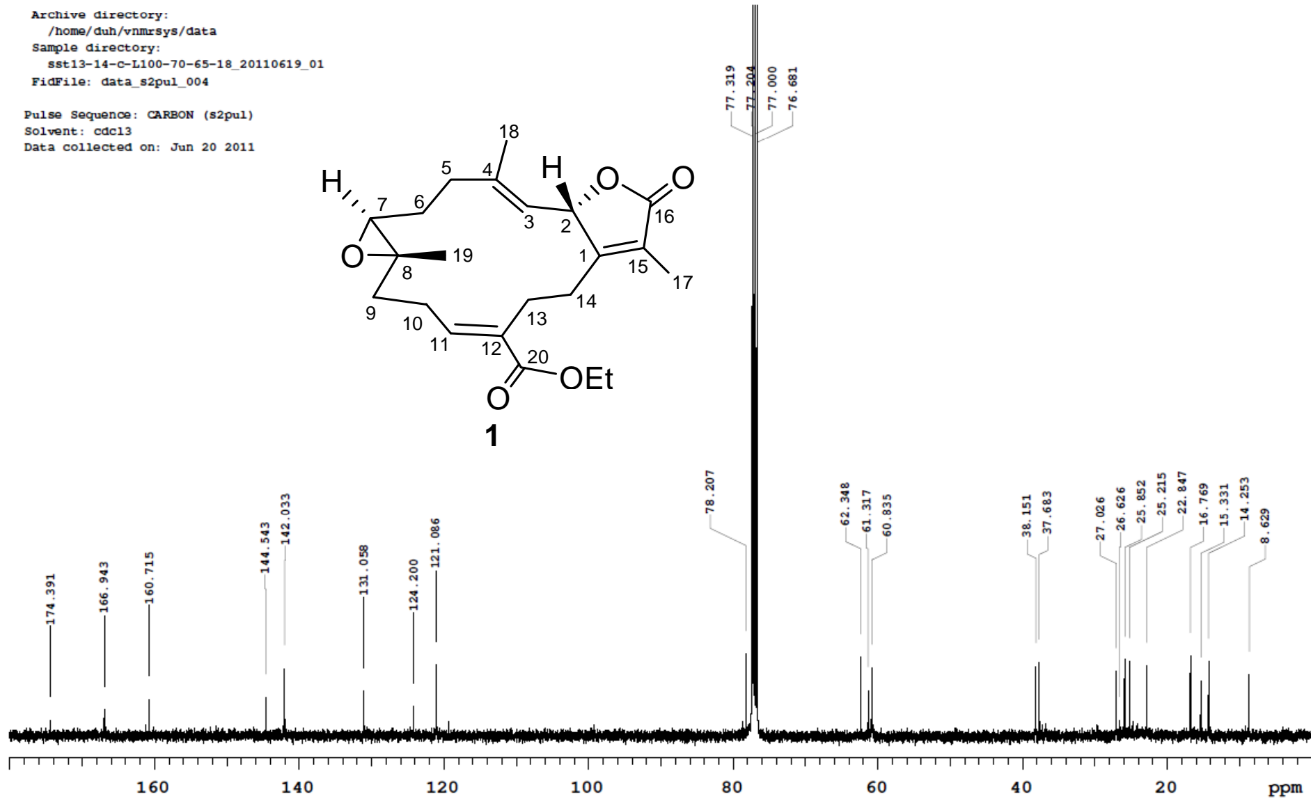
Figure S2. ^{13}\text{C} NMR spectrum (100 MHz) of (+)-12-ethoxycarbonyl-11Z-sarcophine ( 1 ) in \text{CDCl}_3 .
