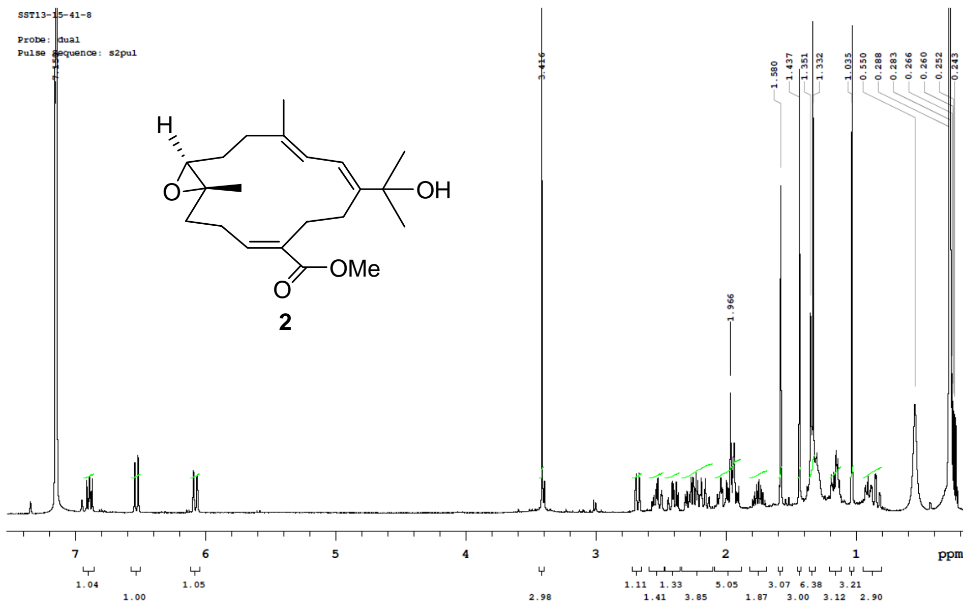
Figure S3. ^1\text{H} NMR spectrum (400 MHz) of ehrenbergol A ( 2 ) in \text{C}_6\text{D}_6 .
