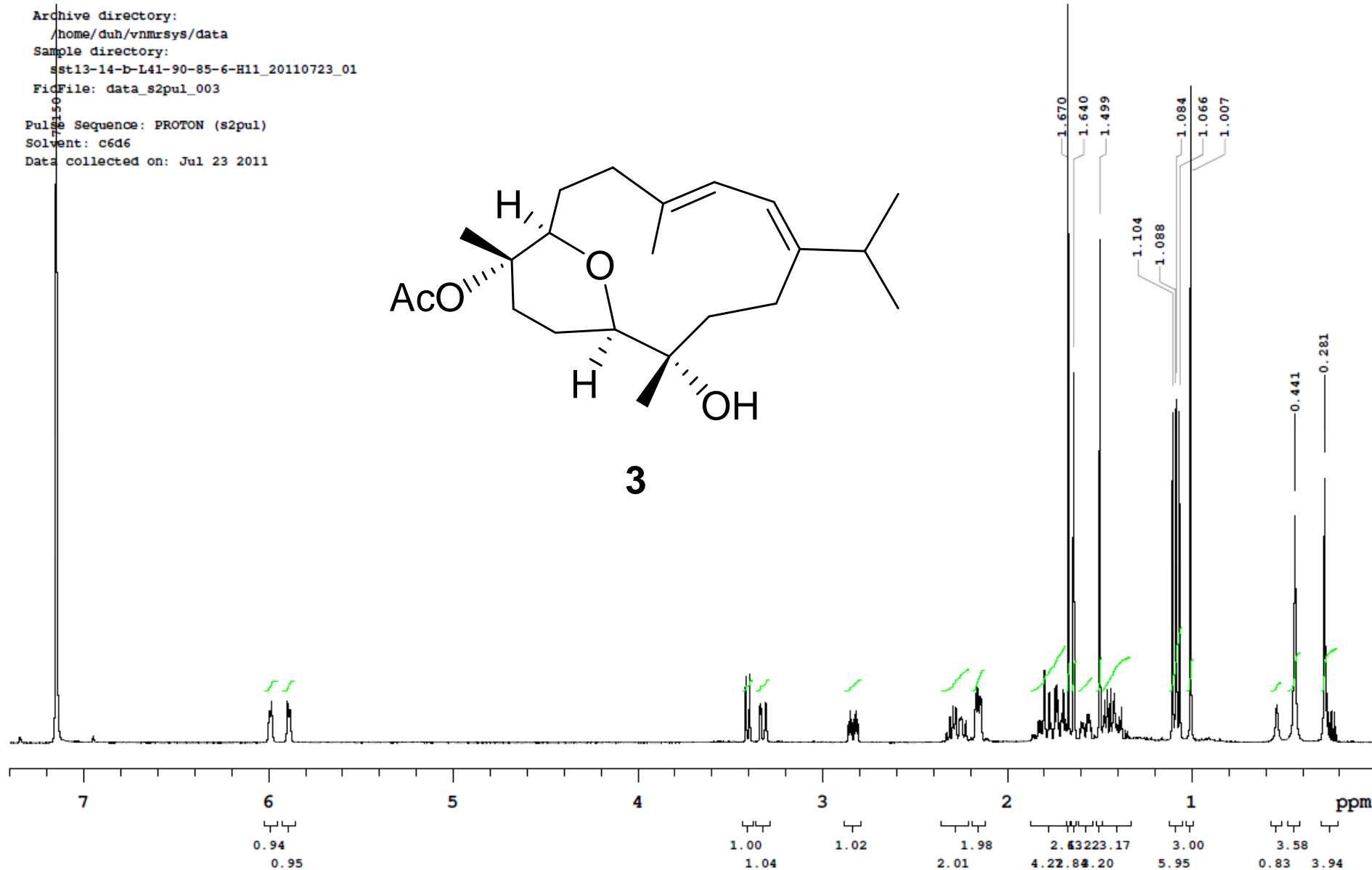
Figure S5. 1 H NMR spectrum (400 MHz) ehrenbergol B (3) in C 6 D 6 .
