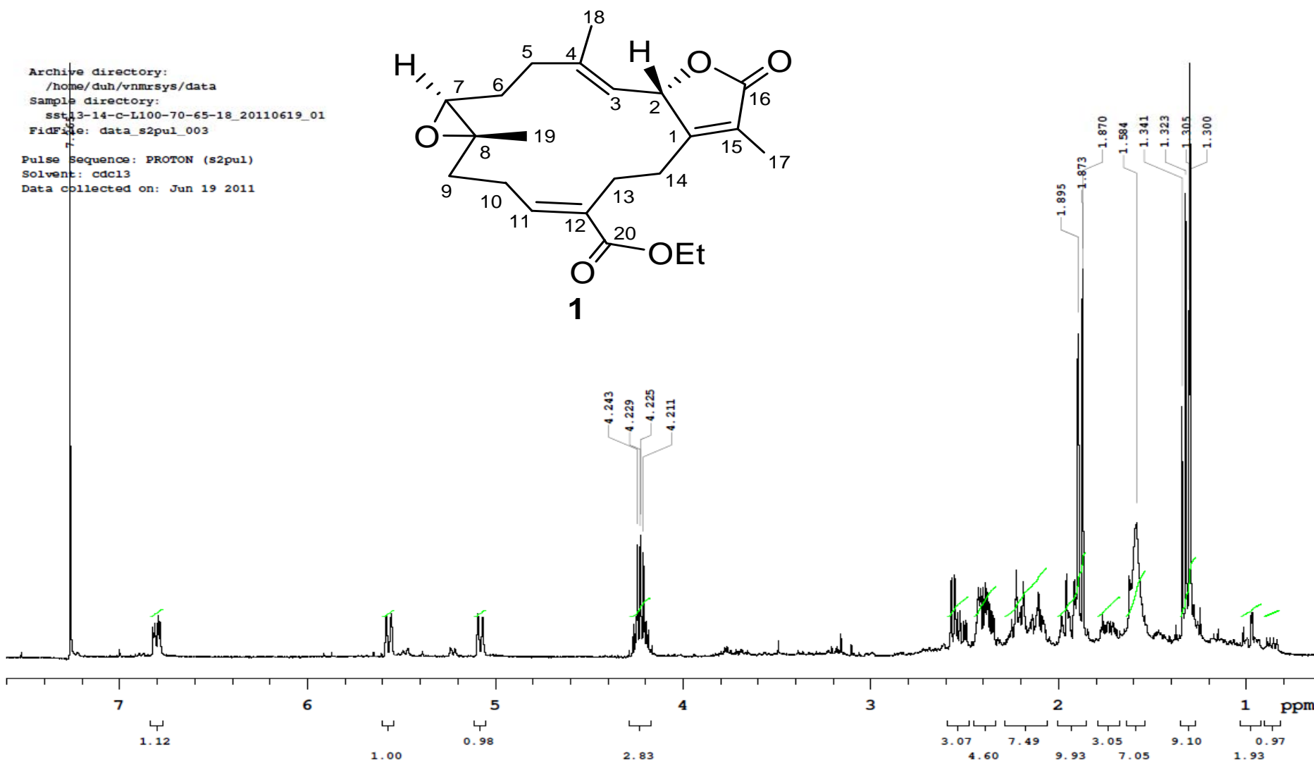
Figure S1. ^1\text{H} NMR spectrum (400 MHz) of (+)-12-ethoxycarbonyl-11Z-sarcophine ( 1 ) in \text{CDCl}_3 .
