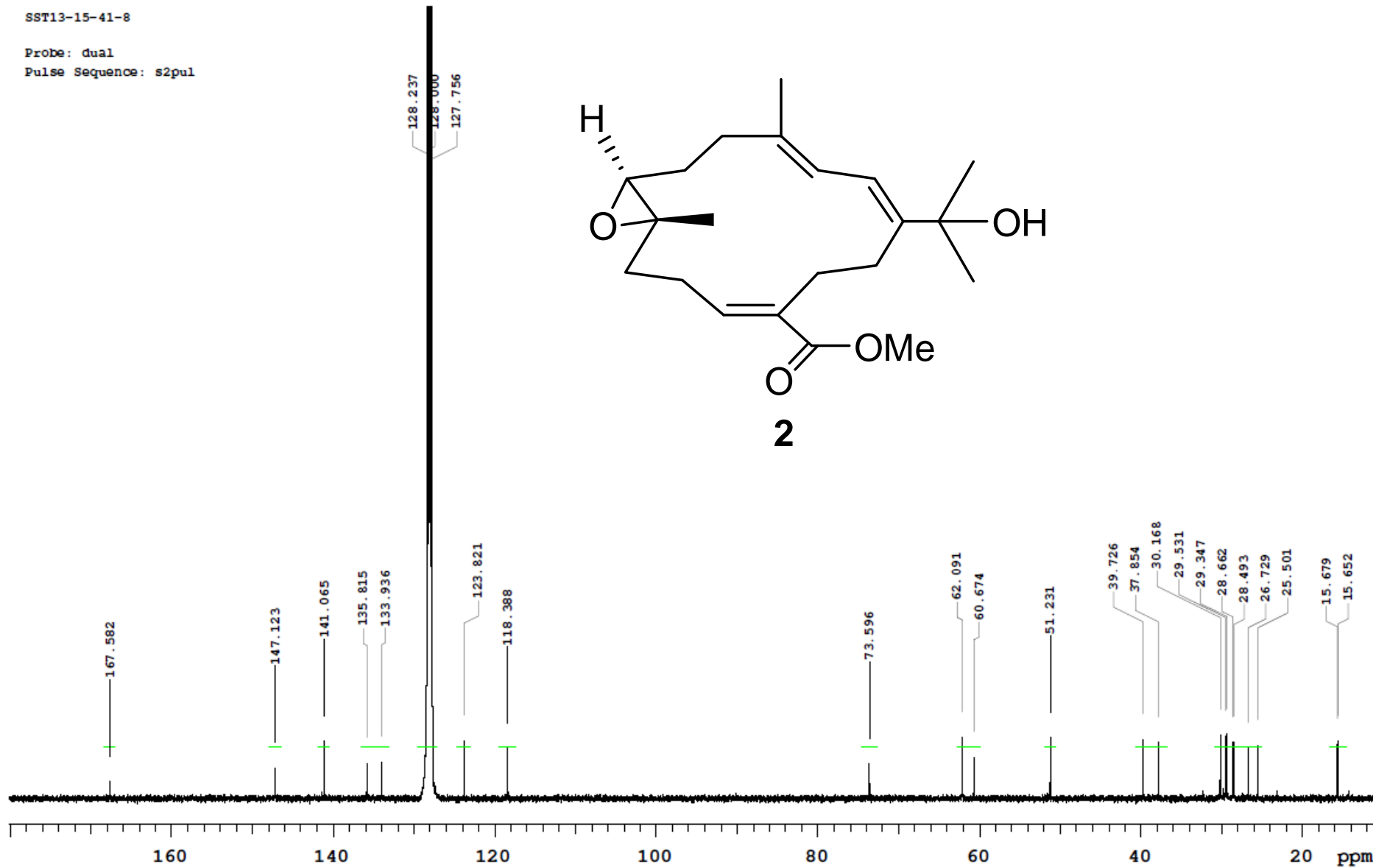
Figure S4. ^{13}\text{C} NMR spectrum (100 MHz) of ehrenbergol A ( 2 ) in \text{C}_6\text{D}_6 .
