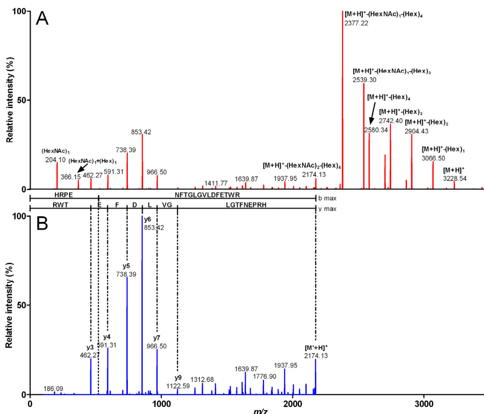
Figure 6. ESI-MS/MS spectra of a glycosylated fragment from Conohyal-Cn1. The ion at m/z 807.8 and corresponding to a 4x-charged species was fragmented by collision-activated dissociation. The singly-charged m/z MS/MS spectrum (A) revealed characteristic signals with mass differences of 162 Da (Hex) and/or 203 Da (HexNAc). Manual interpretation of the spectrum indicated the presence of (HexNAc) 2 (Hex) 4 , information that was used to generate the ESI-MS/MS spectrum in (B) where all Hex-related signals are removed. The final spectrum allowed a correct peptide assignment as the tryptic fragment 104–121.
