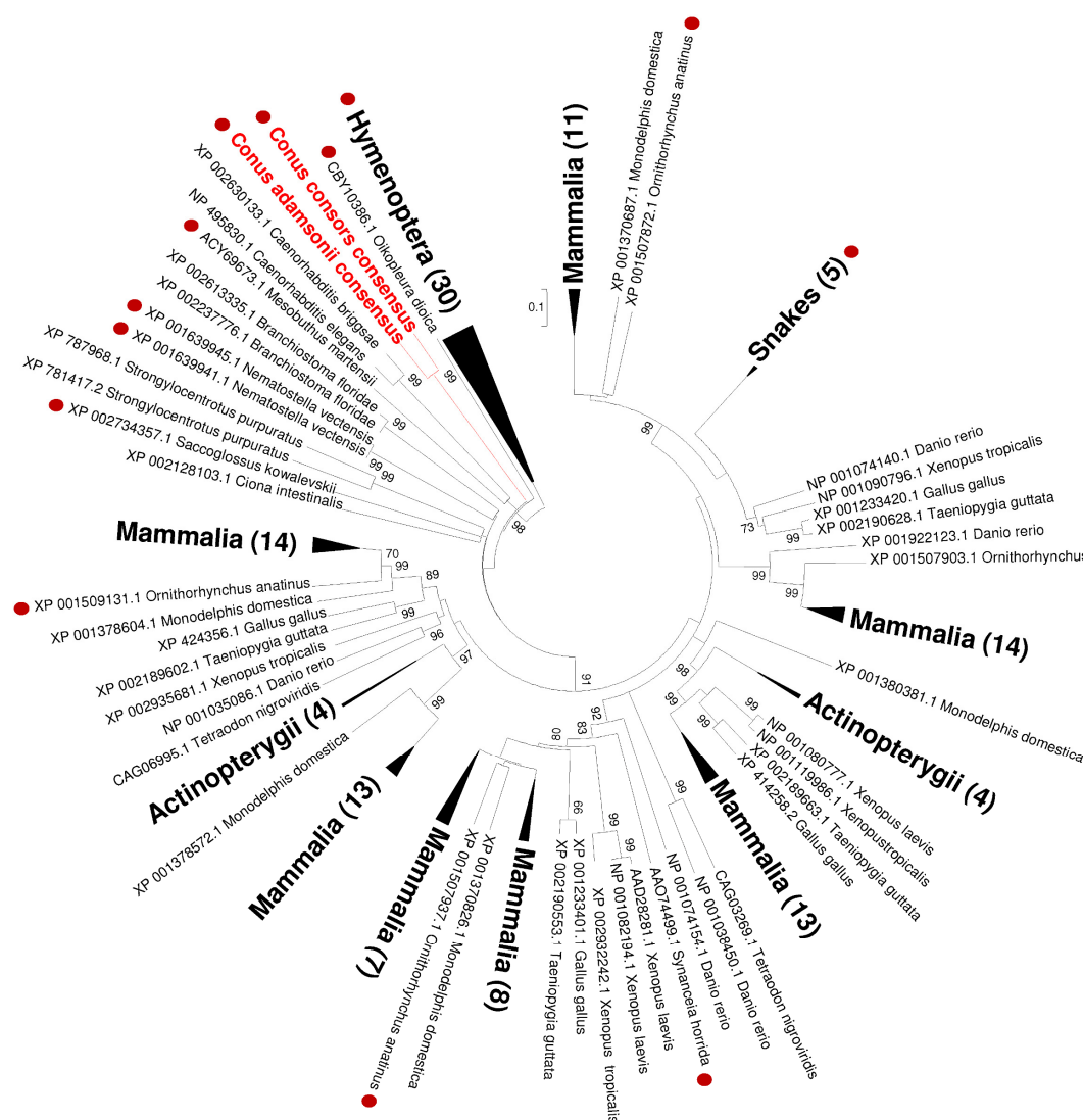
Figure 8. Evolutionary relationships of Hyal sequences using Maximum Likelihood method. Statistically supported clades, including at least five sequences from a monophyletic taxonomic group are collapsed in a same triangle to facilitate tree overview. The surface of each triangle is proportional to the number of sequences in the identified clade. The number of sequences is indicated under the caption of each group. Bootstrap values above 70% are indicated on each node. Outgroup composed by hymenopteran sequences is indicated by a dashed-grey triangle. Sequences are labeled using the Genbank accession number followed by the name of the species. The red dot indicates a putative venom function for a given sequence or in a given clade.
