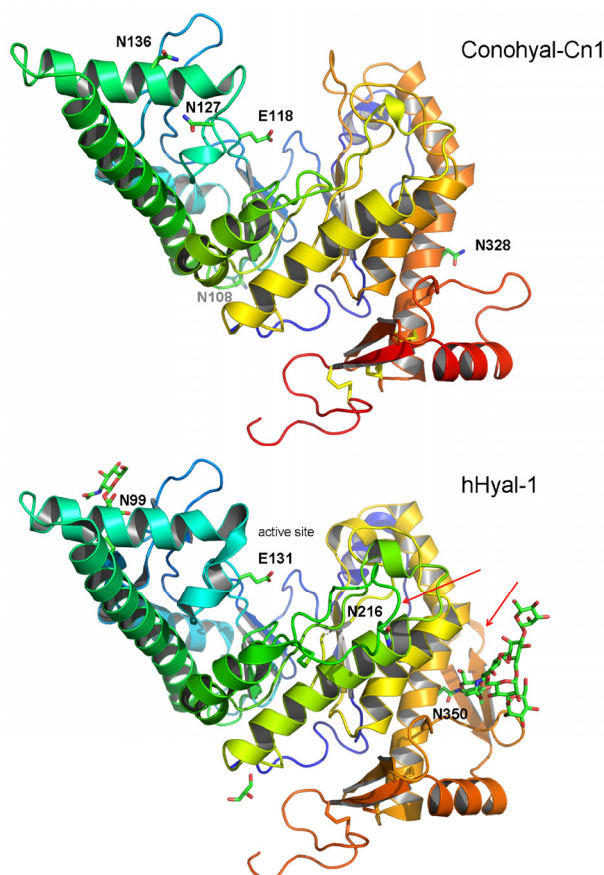
Figure 7. Homology model of Conohyal-Cn1 and X-ray structure of human Hyaluronidase-1 with display of the glycosylation and active sites. Glycosylated position Asn328 in Conohyal-Cn1 is equivalent to Asn350 in hHyal-1. Sugar location in Asn108 for Conohyal-Cn1 has no similarity with the human isoform. Other glycosylation sites include positions Asn127 and/or Asn136 in Conohyal-Cn1 and similarity is shared at position Asn99 for hHyal-1. Spatial position of active sites appears well conserved between the two Hyals. Major structural differences from the homology model of Conohyal-Cn1 and X-ray structure of hHyal-1 are the lack of two loops in Conohyal-Cn1 compared with hHyal-1 (indicated by red arrows, loops 1 and 2).
