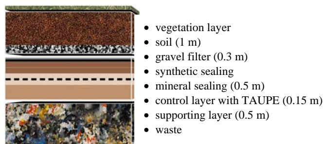
Figure 9. Schematic sketch of a surface barrier system of a waste disposal site.
