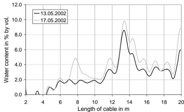
Figure 14. Spatial variation of LWC along the upper horizontal cable at two days during the melting period.
