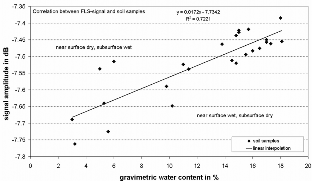
Figure 17. Correlation between the GWC of soil samples and the FLS signal.
