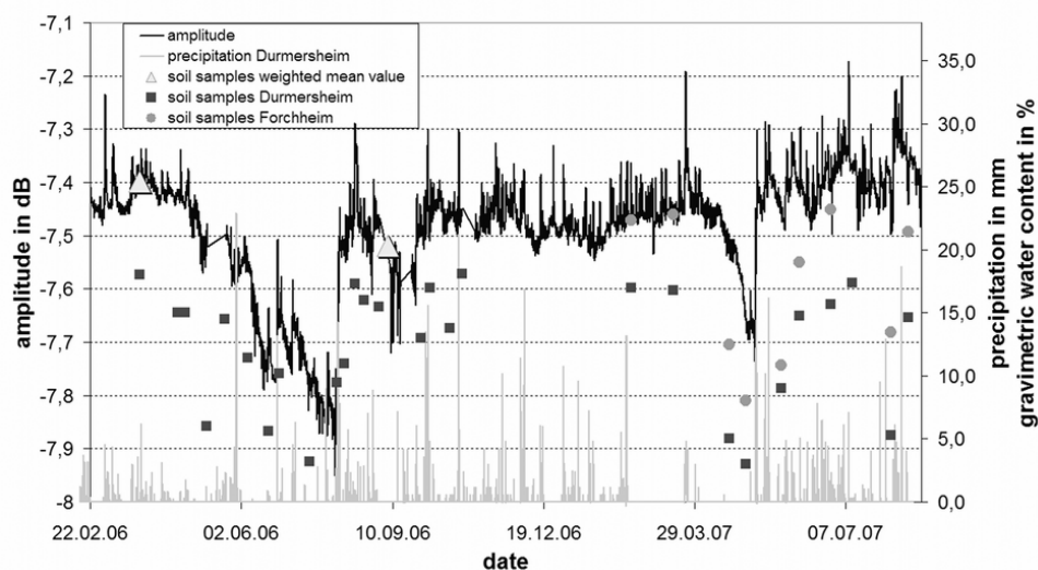
Figure 16. Amplitude of the reflected signal and SM at two sites below the power line. The weighted mean values (triangles) of SM taken along the complete transect are added.
