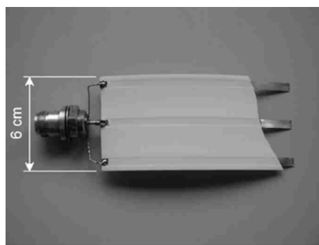
Figure 3. The PE-insulated flat band cable of the TAUPE-TDR sensor. (short section with uncovered conductor to show connection and geometry)
