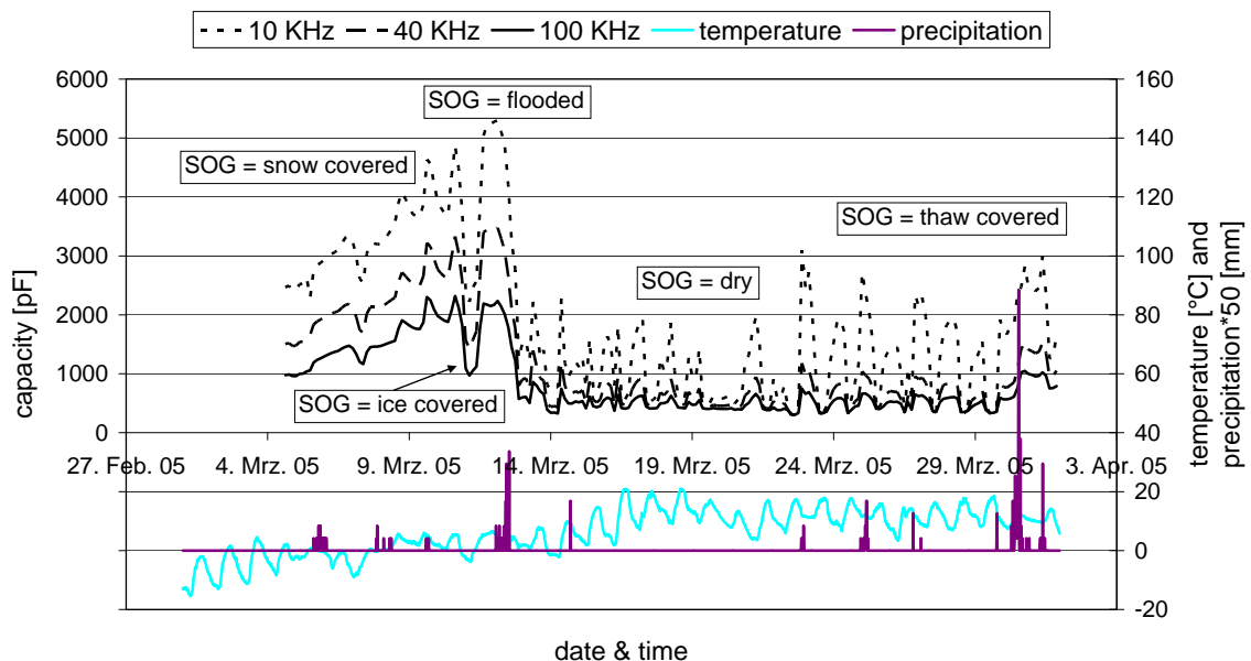
Figure 15. Time-dependent capacities at selected frequencies as well as reference values of temperature and precipitation for different SOG in the month of March 2005.
