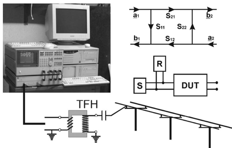
Figure 7. Measuring equipment for the ‘Free Line Sensor’ with a HP3588B vector network analyser, HP35677A S-parameter test set and personal computer. The meaning of the S-parameters is shown on the right; the measuring parameter is the input reflection factor S_{11} = \underline{b}_1 / \underline{a}_1 .
