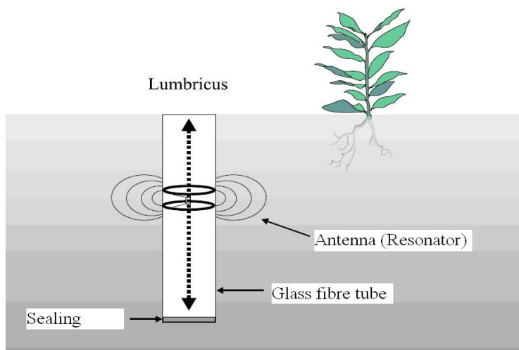
Figure 1. ‘LUMBRICUS’ FD sensor with antenna, access tube and sealing.
