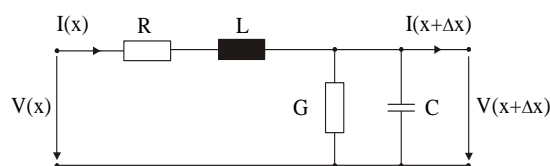
Figure 4. Electric equivalent circuit of an infinitesimal section of a TEM transmission line.
