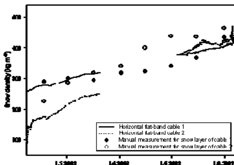
Figure 12. Measurements of snow density as a function of time. Comparison of TAUPE measurements at two different cables with manual measurements with snow cylinder.
