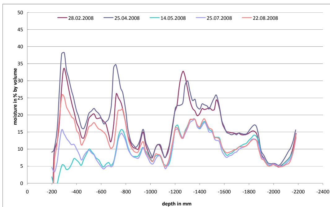
Figure 10. SM depth profiles of a surface barrier of a waste disposal site recorded with LUMBRICUS.
