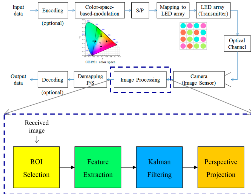
Figure S1. The illustration of LEA detection and tracking method for color-independent visual-MIMO.
