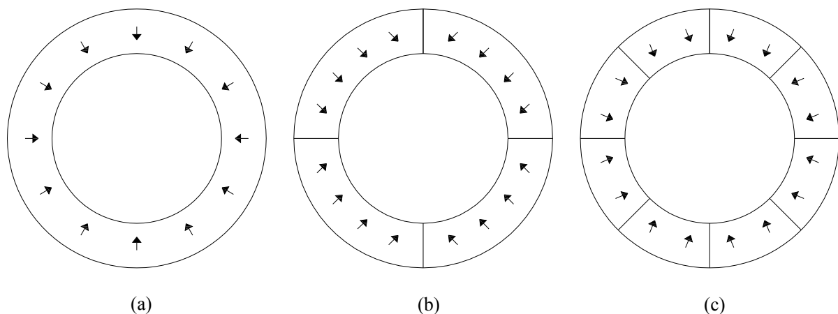
Figure 1. Permanent magnets with (a) ideal radial magnetization; (b) parallel magnetization with four segments forming a ring; and (c) parallel magnetization with eight segments forming a ring.
