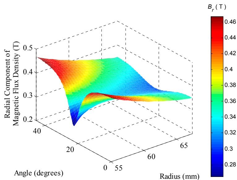
Figure 9. Radial component of magnetic flux density in the region of the coils at a section located at \tau_m/2 of the actuator with ideal radial magnetization.
