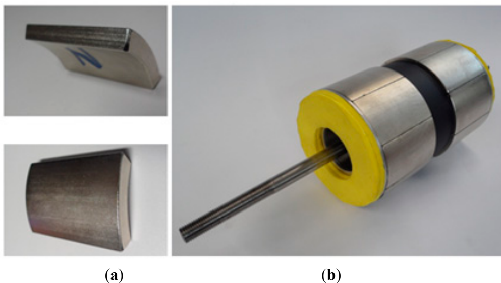
Figure 3. Picture of (a) a 45^\circ segment of magnet with parallel magnetization employed to build the prototype and (b) the mover of the prototype built with two poles of eight segments of permanent magnets with parallel magnetization.
