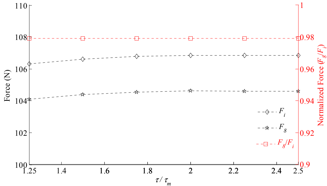
Figure 13. Normalized force ( \tilde{F}_8 = F_8/F_i ) and axial force for an actuator with ideal magnetization ( F_i ) and for an actuator with eight segments with parallel magnetization ( F_8 ) as function of the ratio between permanent magnet length in the axial direction \tau_m and the pole pitch in the axial direction \tau .
