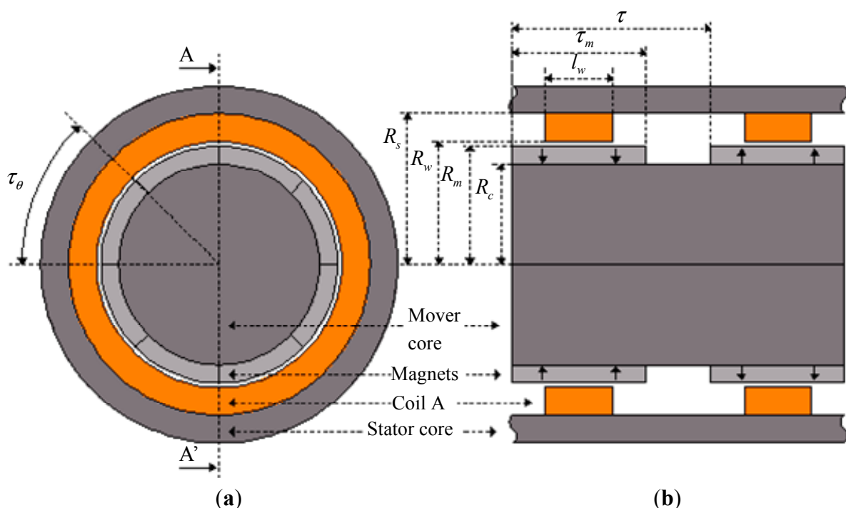
Figure 2. Linear cylindrical actuator showing (a) axial view and (b) view of section AA'.
