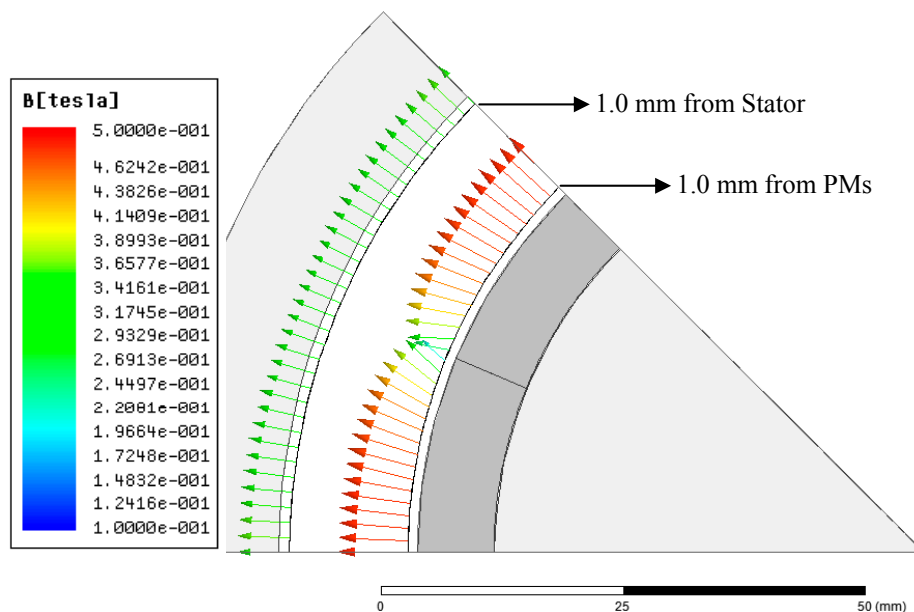
Figure 11. Axial view at \tau_m/2 of the vector B in the air gap at 1.0 mm from the permanent magnets and at 1.0 mm from the stator core.
