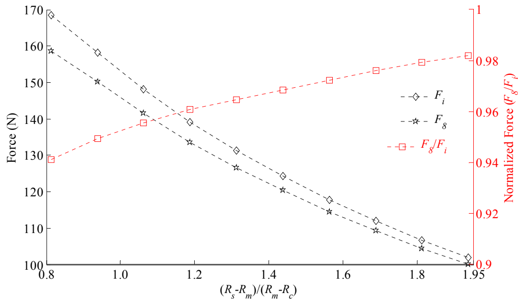
Figure 14. Normalized force ( \tilde{F}_8 = F_8/F_i ) and axial force for an actuator with ideal magnetization ( F_i ) and an actuator with eight segments with parallel magnetization ( F_8 ) as a function of normalized magnetic gap (R_s - R_m)/(R_m - R_c) .
