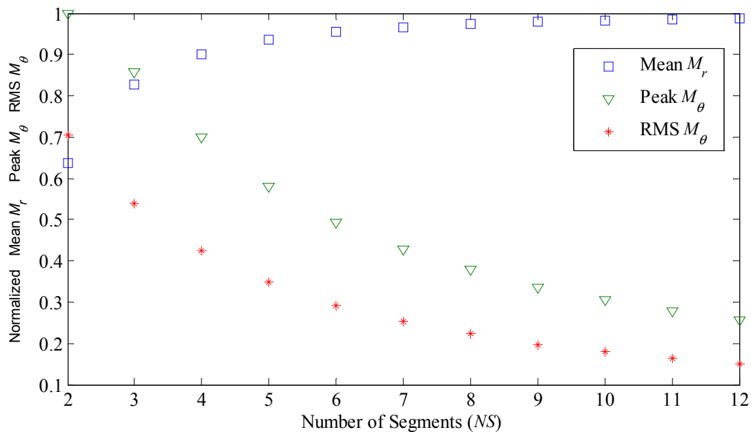
Figure 5. Normalized mean radial component of magnetization for parallel magnetized ring-shaped magnets, and normalized peak value and RMS value of circumferential component for 2 to 12 segments of permanent magnets.
