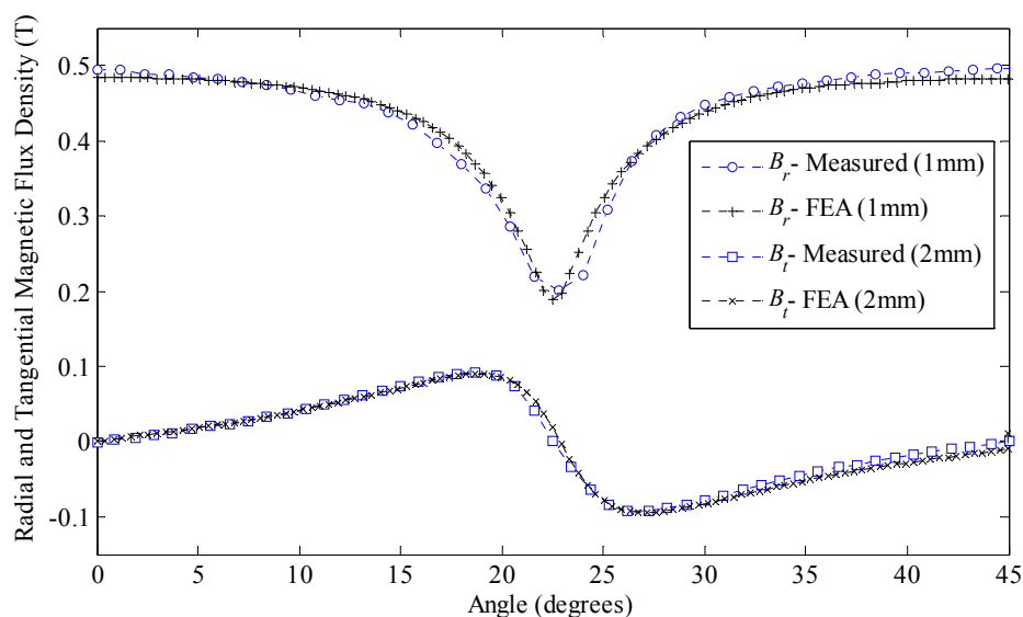
Figure 18. Results of FEA and measurements of normal B_r and tangential B_t components of magnetic flux density as measured in the air gap of the prototype.
