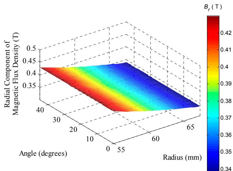
Figure 9. Radial component of magnetic flux density in the region of the coils at a section located at \tau_m/2 of the actuator with ideal radial magnetization.
