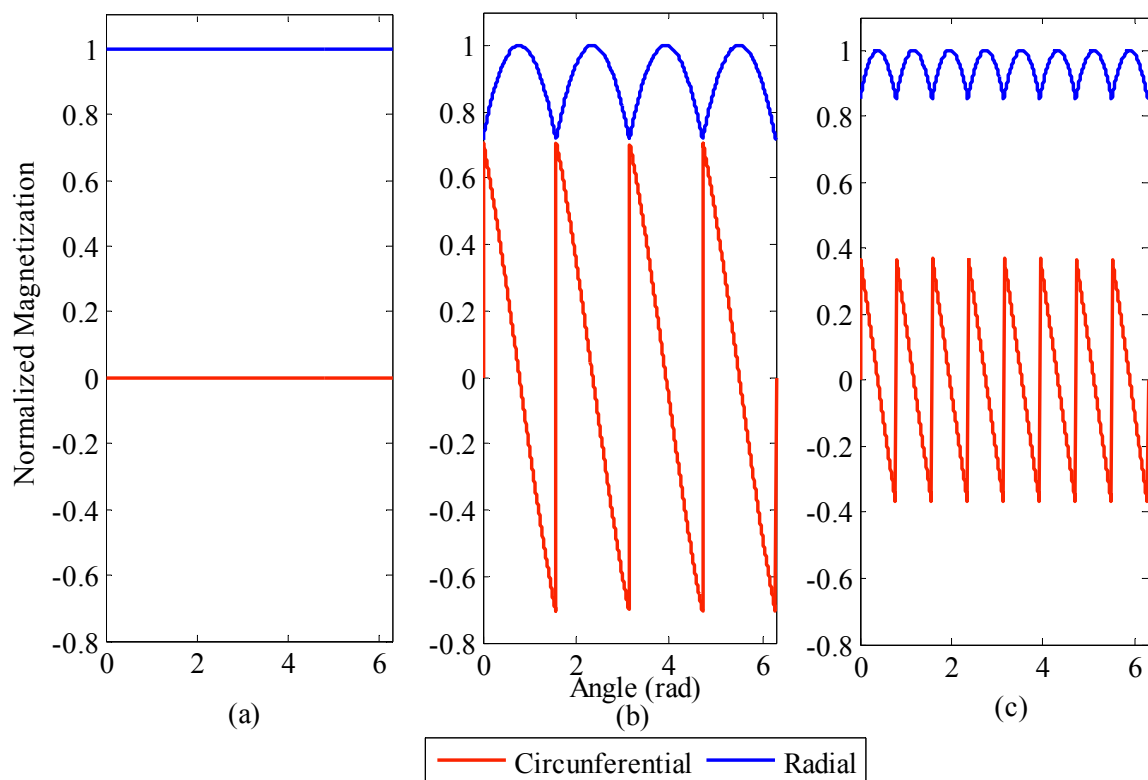
Figure 4. Normalized radial and circumferential magnetization components of ring-shaped magnets with (a) ideal radial magnetization, (b) four segments with parallel magnetization, and (c) eight segments with parallel magnetization.
