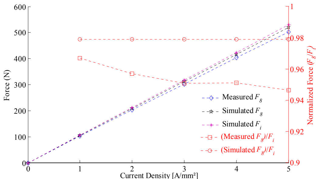
Figure 16. Force versus current density: measured on the prototype (Measured F_8 ) and simulated for an actuator with ideal radial magnetization (Simulated F_i ) and for an actuator with eight segments with parallel magnetization (Simulated F_8 ). Normalized force ((Measured F_8 )/ F_i ) and ((Simulated F_8 )/ F_i ) versus current density.
