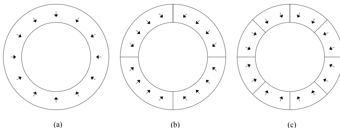
Figure 1. Permanent magnets with (a) ideal radial magnetization; (b) parallel magnetization with four segments forming a ring; and (c) parallel magnetization with eight segments forming a ring.
