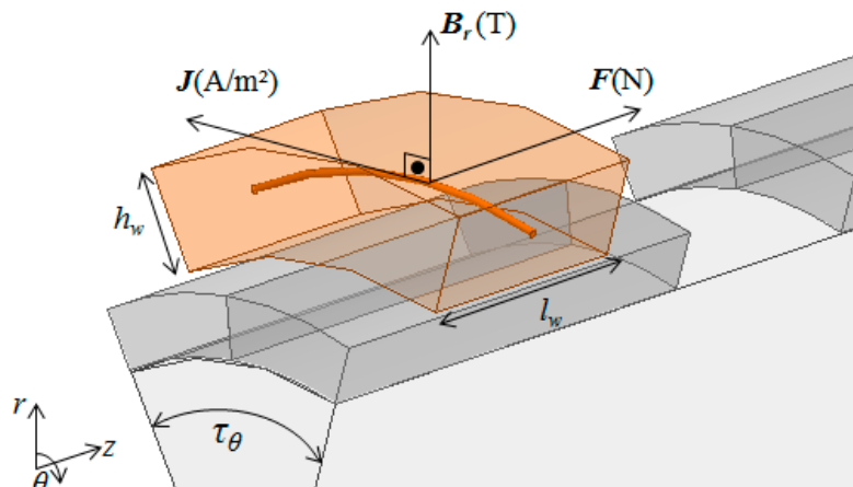
Figure 7. Vectors of radial component of magnetic flux density B_r , electric current density J and force F over a generic electric conductor.
