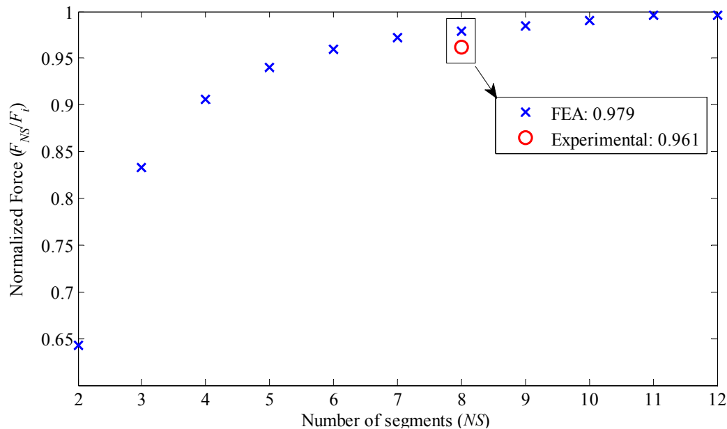
Figure 12. Results of normalized axial force produced by the actuator with parallel magnetized permanent magnets. Values were normalized in relation to an actuator with ideal radial magnetized permanent magnets.
