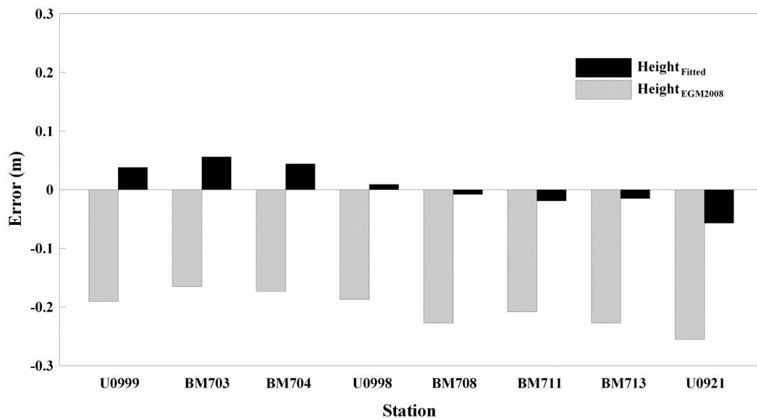
Figure 7. Height accuracy evaluation for Network RTK positioning using EGM2008_{NGA} and EGM2008_{Fitted} applied to the smartphone.
