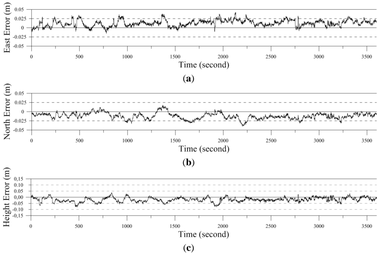
Figure 6. Accuracy test results at UCP U0999 in network RTK positioning: (a) position error for east coordinates; (b) position error for north coordinates; and (c) position error for height coordinates.
