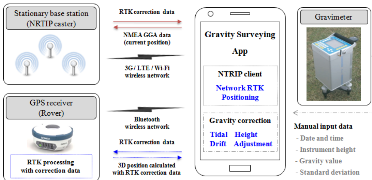
Figure 4. Application design overview consisting of NTRIP client and gravity correction.
