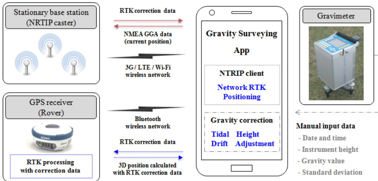
Figure 4. Application design overview consisting of NTRIP client and gravity correction.
