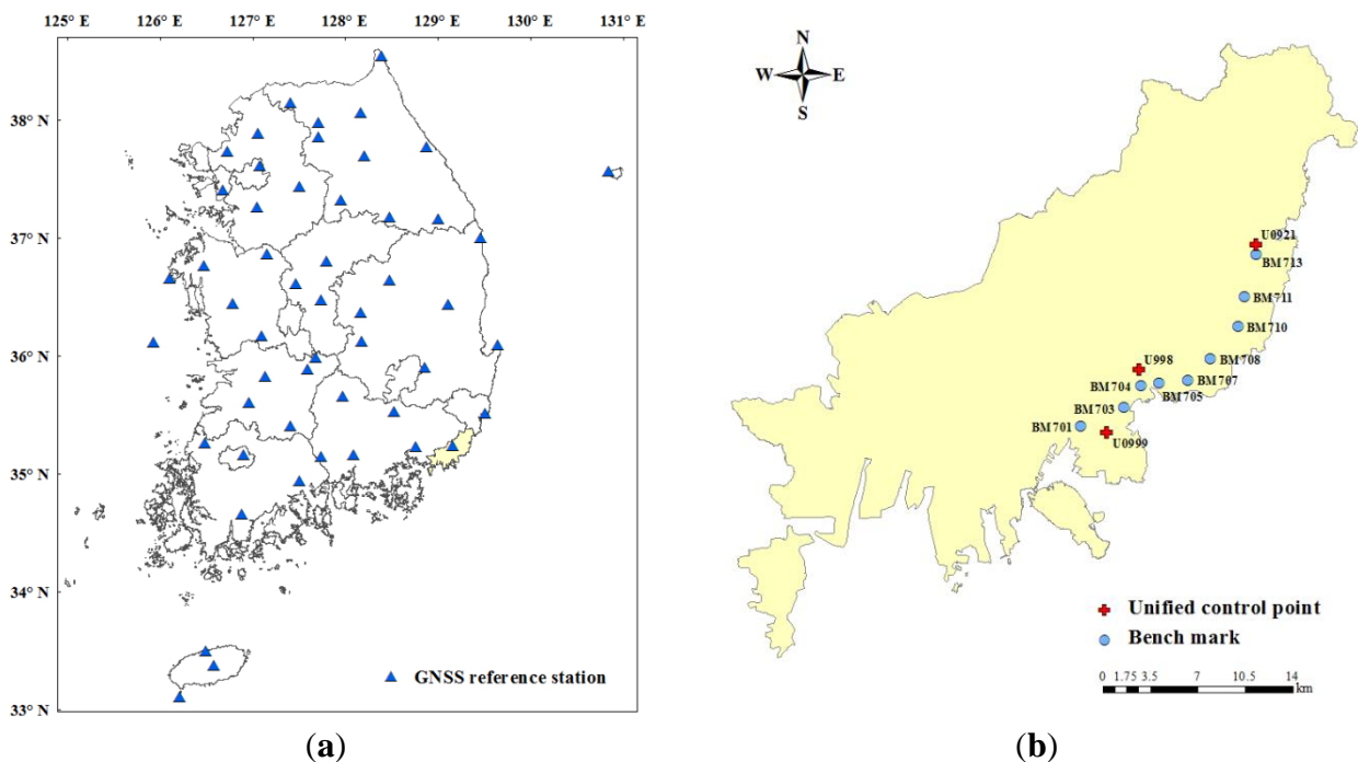
Figure 1. (a) Distribution of 52 GNSS reference stations in South Korea; (b) the study area (three unified control points (UCPs) and eight bench marks (BMs) used in the experiment).
