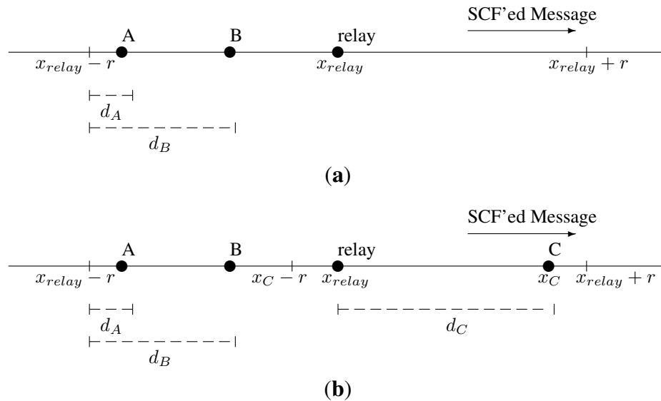
Figure 8. Relay detection in the range [x_{relay} - r, x_{relay} + r] . (a) Equation (9) lets us select B as a new relay; (b) B and C are both selected as new relays. The previous relay must repeat the message from C, so that B can hear it.
