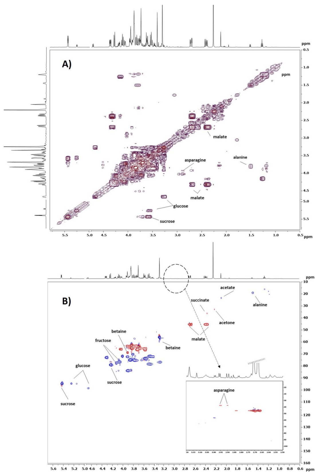
Figure S1. Representative (A) COSY and (B) HSQC spectra of the aqueous extracts of C. coccineum from Sardinia
