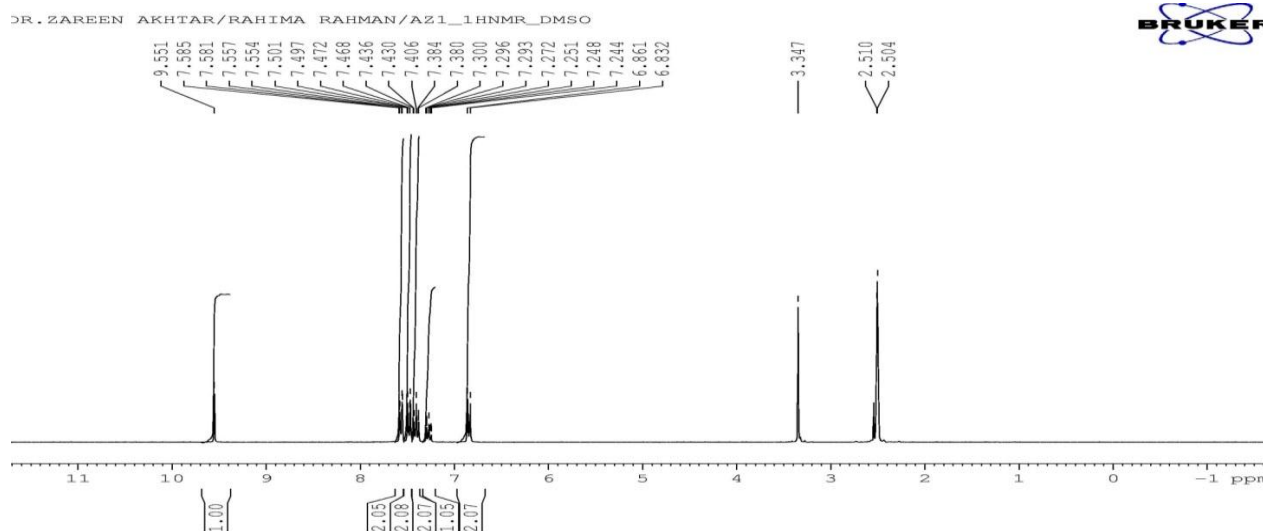
Figure S1. 1 H-NMR spectrum of 4,4'-Bis[4-(4'-hydroxyphenyl)phenylazo]diphenyl Ether.
