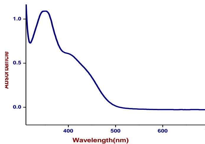
Figure S3. UV-Visible spectrum of 4,4'-Bis[4-(4'-hydroxyphenyl)phenylazo]diphenyl Ether.
