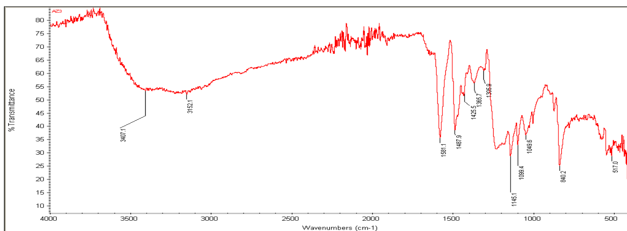
Figure S2. FTIR spectrum of 4,4'-Bis[4-(4'-hydroxyphenyl)phenylazo]diphenyl Ether.
