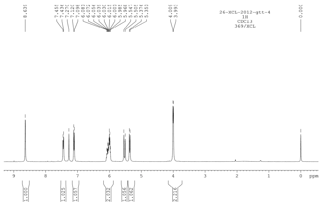
Figure S2. The ^1\text{H} -NMR spectrum of the title compound, 3 .
