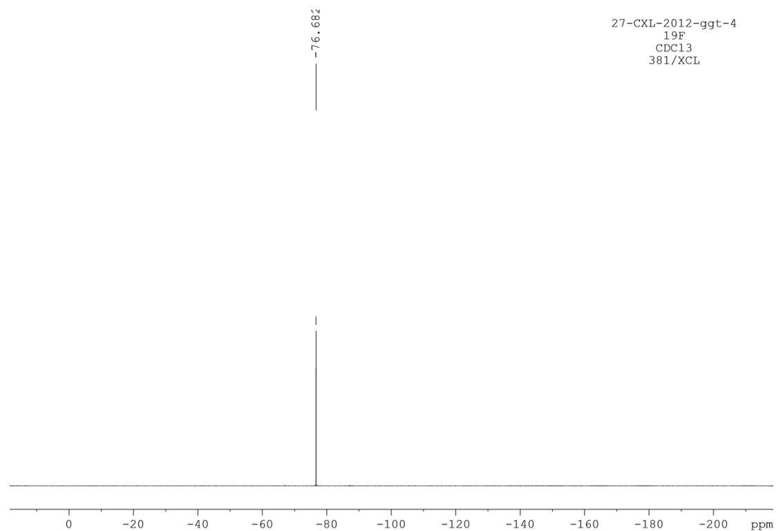
Figure S4. The ^{19}\text{F} -NMR spectrum of the title compound, 3 .
