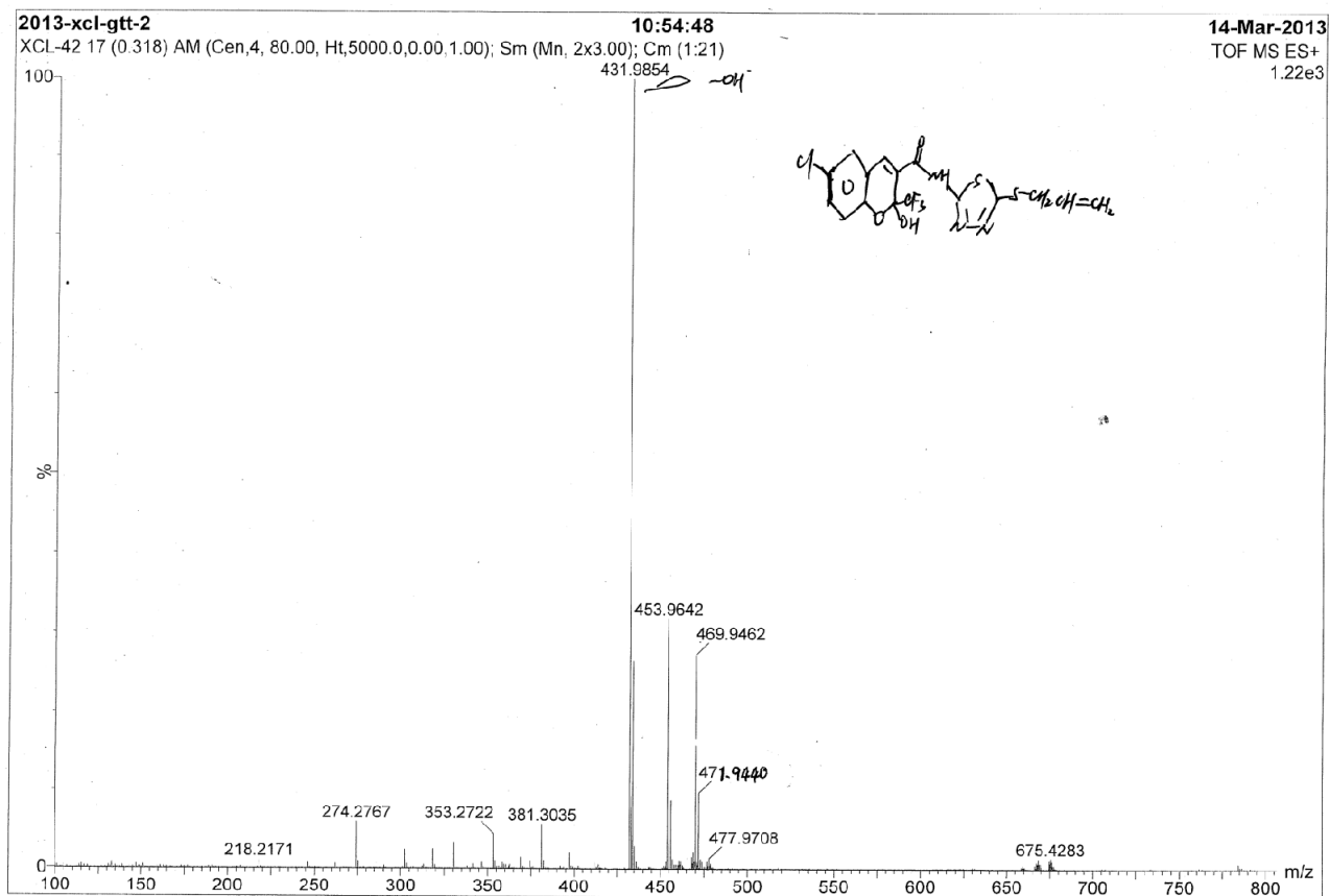
Figure S5. The HRMS spectrum of the title compound, 3 .
