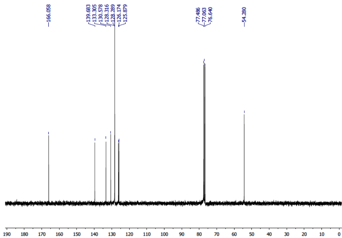
Figure S2. ^{13}\text{C} NMR spectrum of 2 (75 MHz, \text{CDCl}_3 ).
