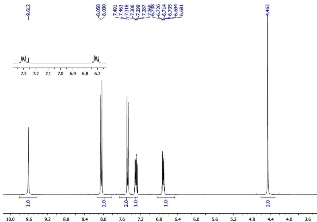
Figure S1. ^1\text{H} NMR spectrum of 2 (300 MHz, \text{CDCl}_3 ).
