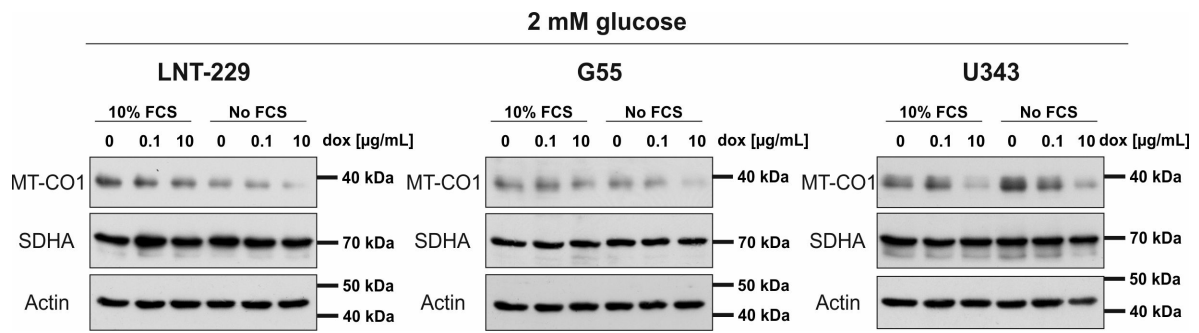
Figure S1: Doxycycline causes mitonuclear protein imbalance in glioma cells under low glucose conditions. LNT-229, G55 and U343 glioma cells were incubated in serum containing (10% FCS) or serum-free (No FCS) medium with glucose restriction (2 mM glucose) with vehicle, 0.1 or 10 \mu g/ml doxycycline under normoxic conditions for 24 h as indicated. Cellular lysates were analyzed by immunoblot with antibodies for MT-CO1, SDHA and actin.
